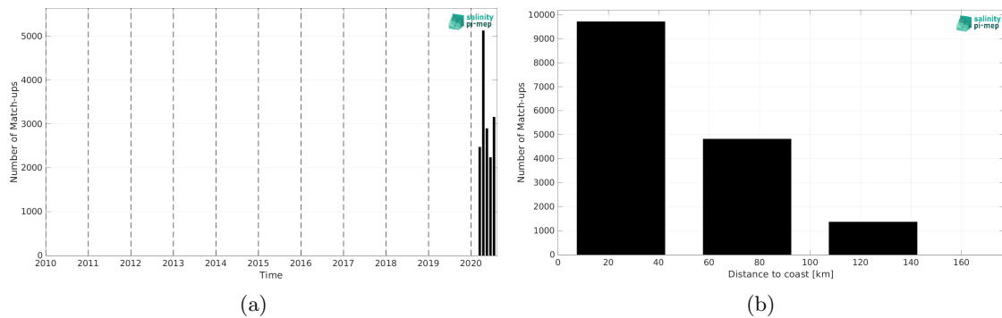
Figure 2: Number of match-ups between Saildrone and SMAP SSS L2 v5.0 (JPL) SSS as a function of time (a) and as function of the distance to coast (b) over the Mediterranean Sea Pi-MEP region and for the full satellite product period.
