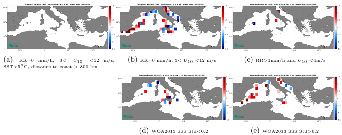
Figure 14: Temporal mean gridded over spatial boxes of size 1^\circ \times 1^\circ of \Delta\text{SSS} (SMAP SSS L2 v5.0 (JPL) - Saldrone) for 5 different subdatasets corresponding to:RR=0 mm/h, 3 < U_{10} < 12 m/s, SST >5^\circ\text{C} , distance to coast > 800 km (a), RR=0 mm/h, 3 < U_{10} < 12 m/s (b), RR >1 mm/h and U_{10} < 4 m/s (c), WOA2013 SSS Std <0.2 (d), WOA2013 SSS Std >0.2 (e).
