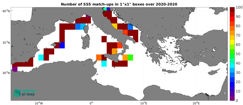
Figure 5: Number of SSS match-ups between Saildrone SSS and the SMAP SSS L2 v5.0 (JPL) SSS product for the Mediterranean Sea Pi-MEP region over 1^\circ \times 1^\circ boxes and for the full satellite product period.
