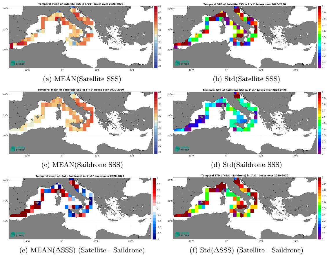
Figure 6: Temporal mean (left) and Std (right) of SSS from SMAP SSS L2 v5.0 (JPL) (top), Saildrone (middle), and of \Delta SSS (Satellite - Saildrone). Only match-up pairs are used to generate these maps.
