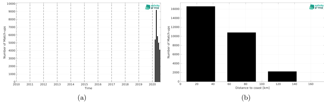
Figure 1: Number of match-ups between Sairdrone and SMAP SSS L2 v5.0 (JPL) SSS as a function of time (a) and as function of the distance to coast (b) over the Mediterranean Sea Pi-MEP region and for the full satellite product period.
