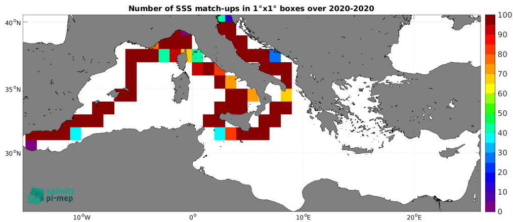
Figure 4: Number of SSS match-ups between Saildrone SSS and the SMAP SSS L2 v5.0 (JPL) SSS product for the Mediterranean Sea Pi-MEP region over 1^\circ \times 1^\circ boxes and for the full satellite product period.
