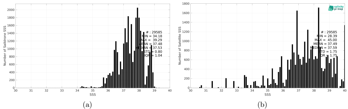
Figure 2: Histograms of SSS from Sairdrone (a) and SMAP SSS L2 v5.0 (JPL) (b) considering all match-up pairs per bins of 0.1 over the Mediterranean Sea Pi-MEP region and for the full satellite product period.
