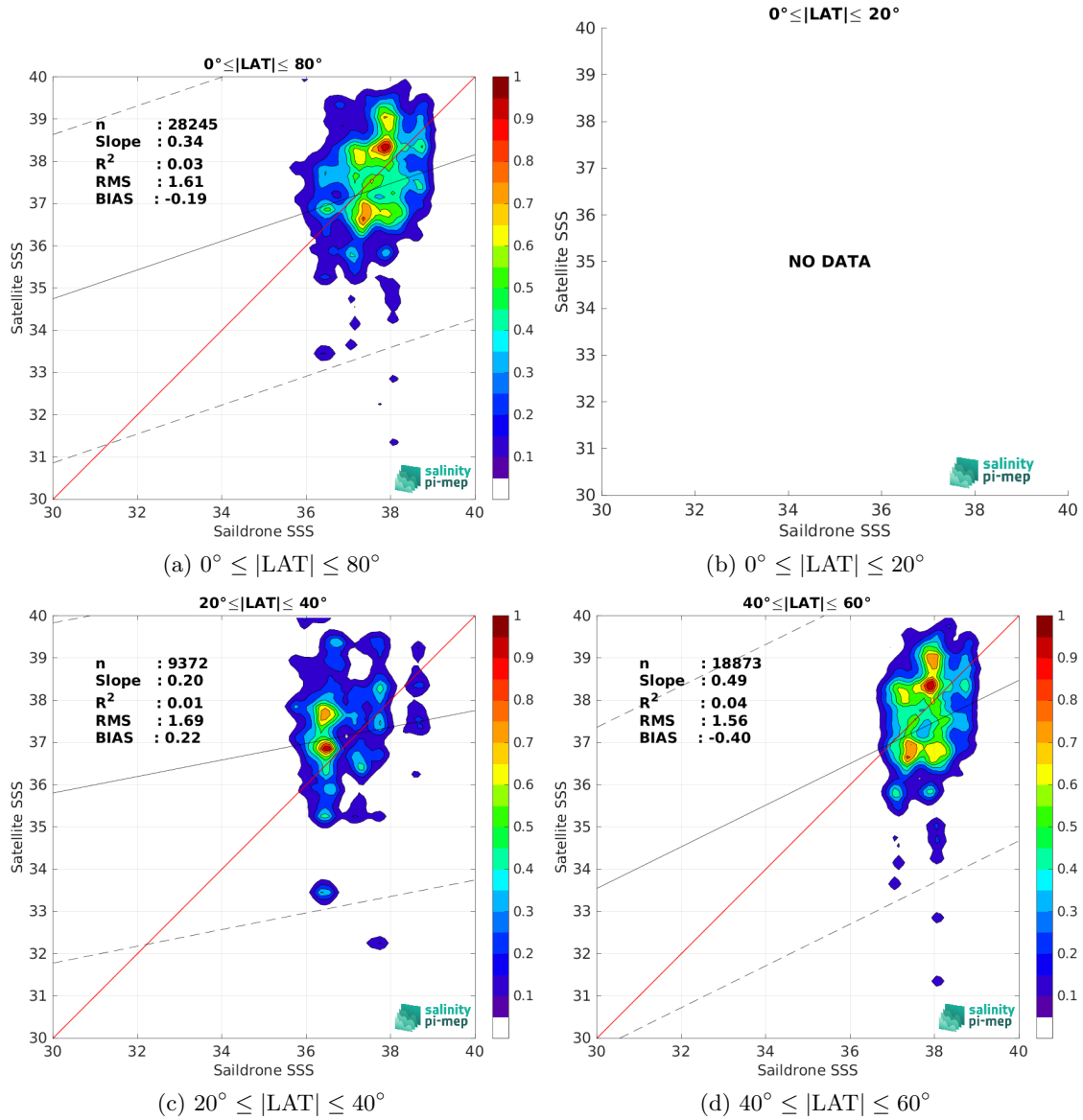
Figure 9: Contour maps of the concentration of SMAP SSS L2 v5.0 (JPL) SSS (y-axis) versus Saildrone SSS (x-axis) at match-up pairs for different latitude bands. For each plot, the red line shows x=y . The black thin and dashed lines indicate a linear fit through the data cloud and the \pm 95\% confidence levels, respectively. The number match-up pairs n , the slope and R^2 coefficient of the linear fit, the root mean square (RMS) and the mean bias between satellite and in situ data are indicated for each latitude band in each plots.
