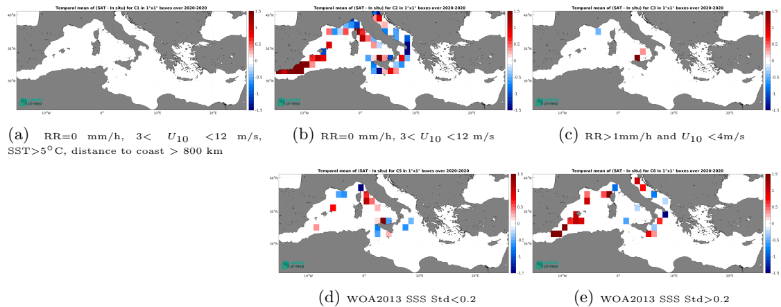
Figure 12: Temporal mean gridded over spatial boxes of size 1^\circ \times 1^\circ of \Delta SSS (SMAP SSS L2 v5.0 (JPL) - Saldrone) for 5 different subdatasets corresponding to:RR=0 mm/h, 3 < U_{10} < 12 m/s, SST >5^\circ\text{C} , distance to coast > 800 km (a), RR=0 mm/h, 3 < U_{10} < 12 m/s (b), RR >1 mm/h and U_{10} < 4 m/s (c), WOA2013 SSS Std <0.2 (d), WOA2013 SSS Std >0.2 (e).
