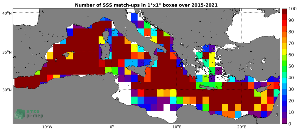
Figure 4: Number of SSS match-ups between Argo SSS and the SMAP SSS L2 v5.0 (JPL) SSS product for the Mediterranean Sea Pi-MEP region over 1°x1° boxes and for the full satellite product period.
