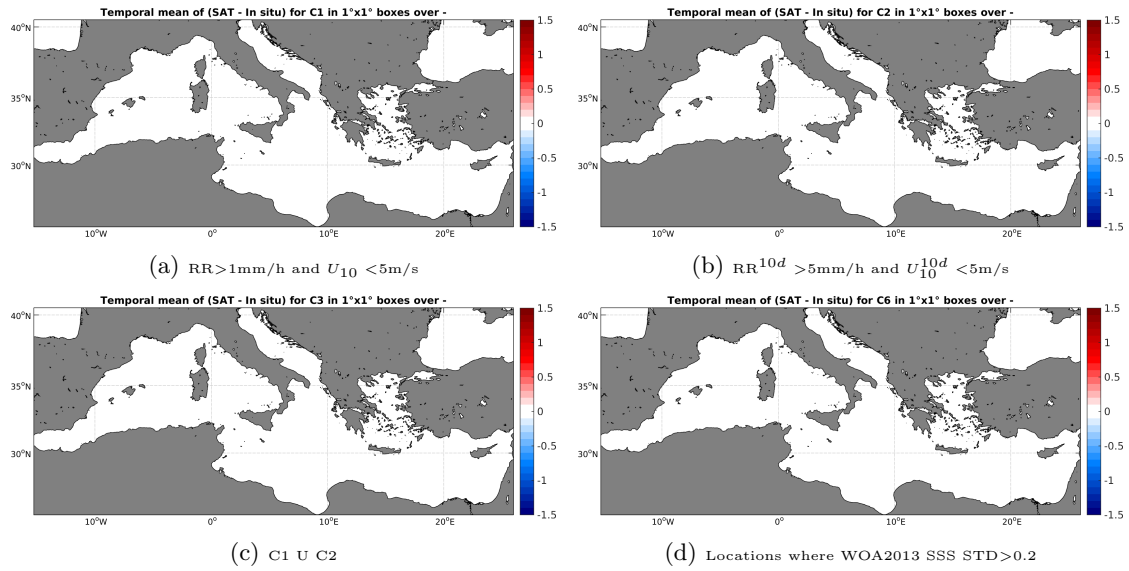
Figure 12: Temporal mean gridded over spatial boxes of size 1^\circ \times 1^\circ of \Delta SSS (SMAP-L2-JPL-V4 - TSG-SAMOS) for 4 different subdatasets corresponding to: RR > 1\text{mm/h} and U_{10} < 5\text{m/s} (a), RR^{10d} > 5\text{mm/h} and U_{10}^{10d} < 5\text{m/s} (b), C1 \cup C2 (c), Locations where WOA2013 SSS STD > 0.2 (d).
