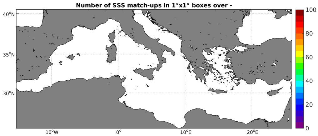
Figure 4: Number of SSS match-ups between TSG-SAMOS SSS and the SMAP-L2-JPL-V4 SSS product for the Mediterranean Sea Pi-MEP region over 1^\circ \times 1^\circ boxes and for the full satellite product period.
