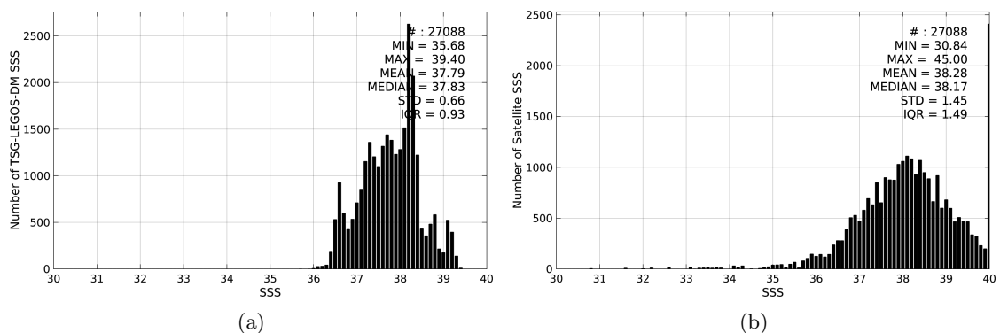
Figure 2: Histograms of SSS from TSG-LEGOS-DM (a) and SMAP-L2-JPL-V4 (b) considering all match-up pairs per bins of 0.1 over the Mediterranean Sea Pi-MEP region and for the full satellite product period.
