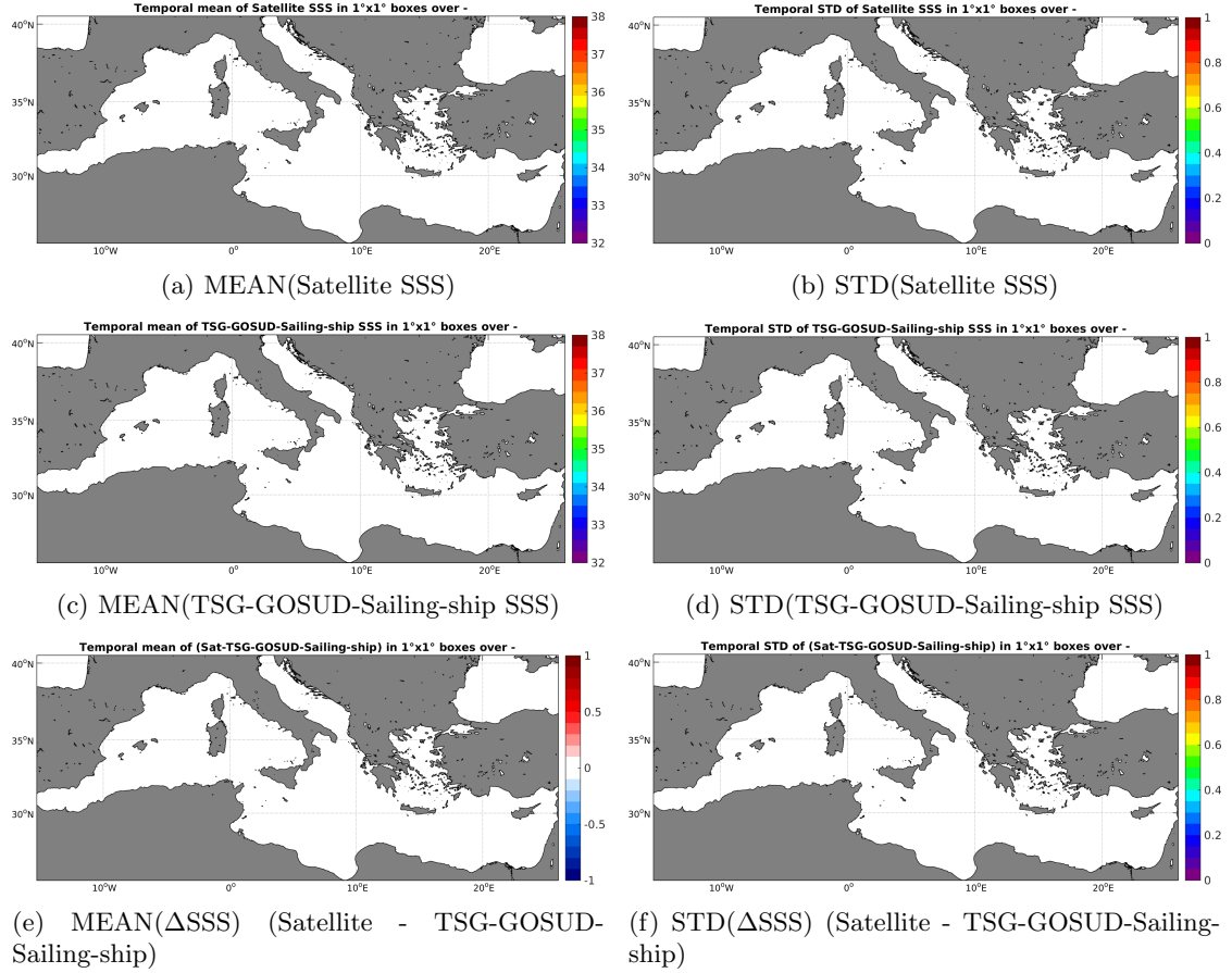
Figure 6: Temporal mean (left) and STD (right) of SSS from SMAP-L2-JPL-V4 (top), TSG-GOSUD-Sailing-ship (middle), and of \Delta SSS (Satellite - TSG-GOSUD-Sailing-ship). Only match-up pairs are used to generate these maps.
