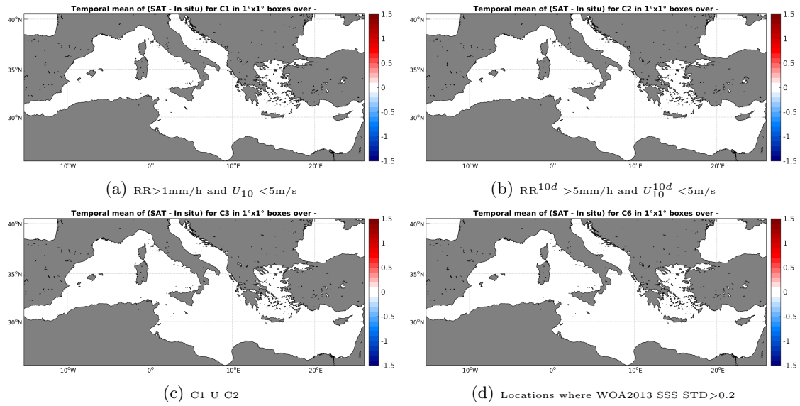
Figure 12: Temporal mean gridded over spatial boxes of size 1^\circ \times 1^\circ of \Delta SSS (SMAP-L2-JPL-V4 - TSG-GOSUD-Sailing-ship) for 4 different subdatasets corresponding to:RR >1 mm/h and U_{10} < 5 m/s (a), RR ^{10d} > 5 mm/h and U_{10}^{10d} < 5 m/s (b), C1 U C2 (c),Locations where WOA2013 SSS STD >0.2 (d).
