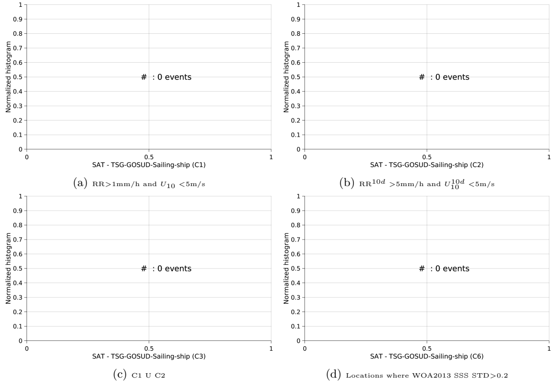
Figure 13: Normalized histogram of \Delta\text{SSS} (SMAP-L2-JPL-V4 - TSG-GOSUD-Sailing-ship) for 6 different subdatasets corresponding to: RR > 1\text{mm/h} and U_{10} < 5\text{m/s} (a), RR^{10d} > 5\text{mm/h} and U_{10}^{10d} < 5\text{m/s} (b), C1 U C2 (c), Locations where WOA2013 SSS STD > 0.2 (d).
