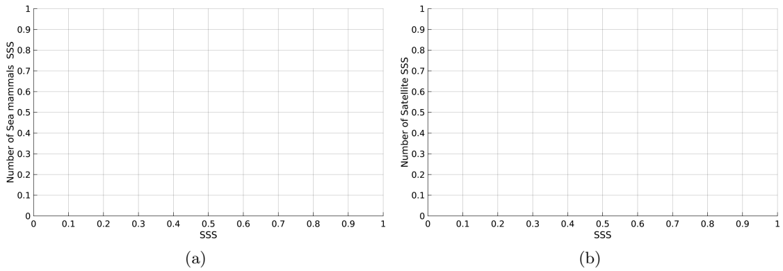
Figure 2: Histograms of SSS from Sea mammals (a) and SMAP-L2-JPL-V4 (b) considering all match-up pairs per bins of 0.1 over the Mediterranean Sea Pi-MEP region and for the full satellite product period.
