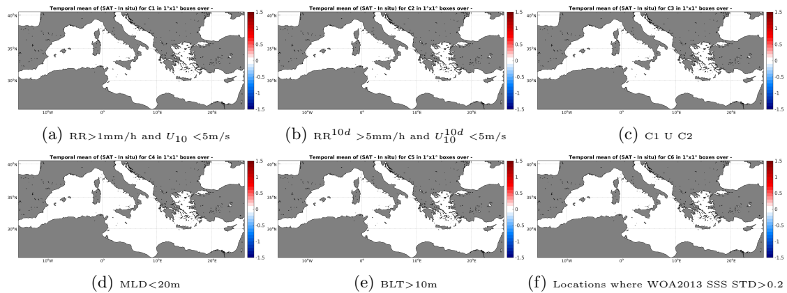
Figure 12: Temporal mean gridded over spatial boxes of size 1^\circ \times 1^\circ of \Delta SSS (SMAP-L2-JPL-V4 - Sea mammals) for 6 different subdatasets corresponding to: RR > 1\text{mm/h} and U_{10} < 5\text{m/s} (a), RR^{10d} > 5\text{mm/h} and U_{10}^{10d} < 5\text{m/s} (b), C1 U C2 (c), MLD < 20\text{m} (d), BLT > 10\text{m} (e), Locations where WOA2013 SSS STD > 0.2 (f).
