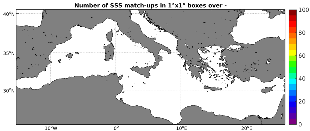
Figure 3: Number of SSS match-ups between Surface drifters SSS and the SMAP-L2-JPL-V4 SSS product for the Mediterranean Sea Pi-MEP region over 1^\circ \times 1^\circ boxes and for the full satellite product period.
