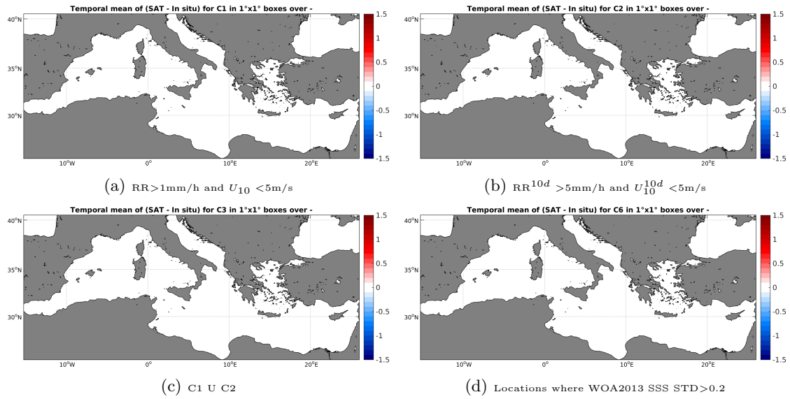
Figure 11: Temporal mean gridded over spatial boxes of size 1^\circ \times 1^\circ of \Delta SSS (SMAP-L2-JPL-V4 - Surface drifters) for 4 different subdatasets corresponding to: RR > 1\text{mm/h} and U_{10} < 5\text{m/s} (a), RR^{10d} > 5\text{mm/h} and U_{10}^{10d} < 5\text{m/s} (b), C1 U C2 (c), Locations where WOA2013 SSS STD > 0.2 (d).
