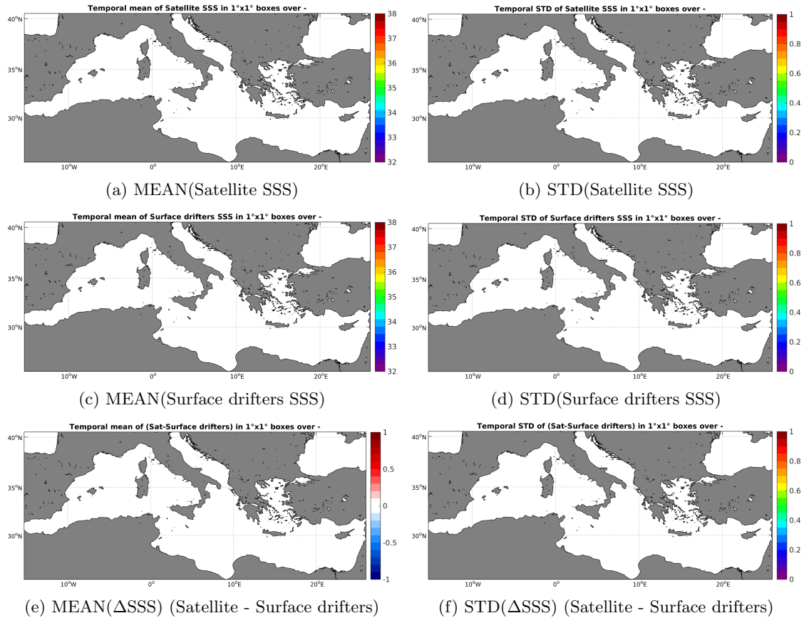
Figure 5: Temporal mean (left) and STD (right) of SSS from SMAP-L2-JPL-V4 (top), Surface drifters (middle), and of \Delta SSS (Satellite - Surface drifters). Only match-up pairs are used to generate these maps.
