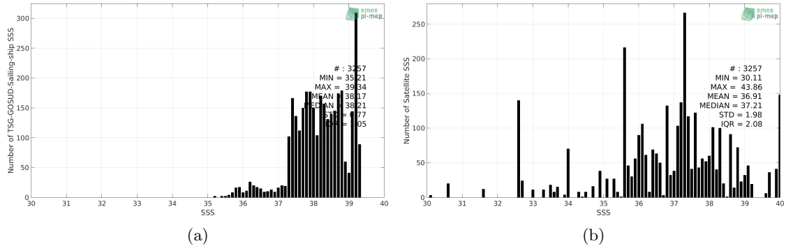
Figure 2: Histograms of SSS from TSG-GOSUD-Sailing-ship (a) and SMAP-L2-JPL-V4.3 (b) considering all match-up pairs per bins of 0.1 over the Mediterranean Sea Pi-MEP region and for the full satellite product period.
