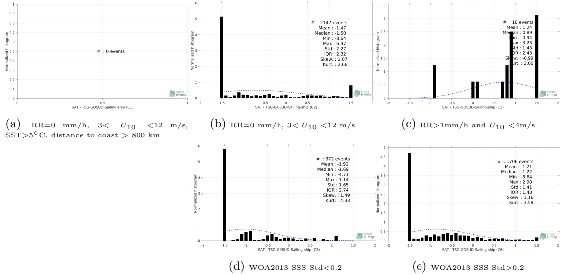
Figure 13: Normalized histogram of \Delta\text{SSS} (SMAP-L2-JPL-V4.3 - TSG-GOSUD-Sailing-ship) for 5 different subdatasets corresponding to: RR=0 mm/h, 3 < U_{10} < 12 m/s, SST > 5^\circ\text{C} , distance to coast > 800 km (a), RR=0 mm/h, 3 < U_{10} < 12 m/s (b), RR > 1\text{mm/h} and U_{10} < 4\text{m/s} (c), WOA2013 SSS Std < 0.2 (d), WOA2013 SSS Std > 0.2 (e).
