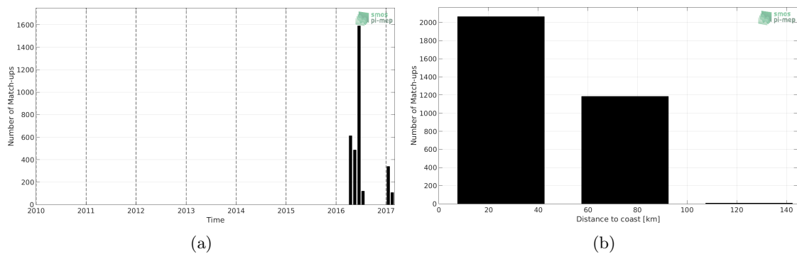
Figure 1: Number of match-ups between TSG-GOSUD-Sailing-ship and SMAP-L2-JPL-V4.3 SSS as a function of time (a) and as function of the distance to coast (b) over the Mediterranean Sea Pi-MEP region and for the full satellite product period.
