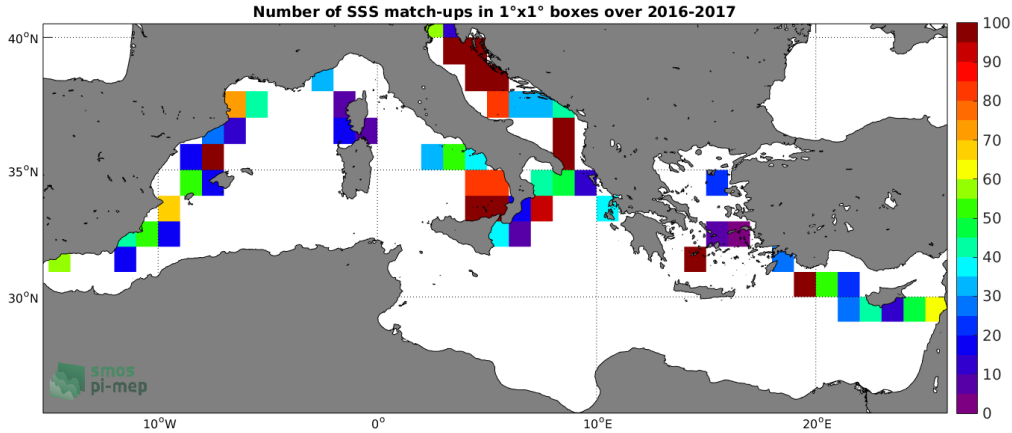
Figure 4: Number of SSS match-ups between TSG-GOSUD-Sailing-ship SSS and the SMAP-L2-JPL-V4.3 SSS product for the Mediterranean Sea Pi-MEP region over 1^\circ \times 1^\circ boxes and for the full satellite product period.
