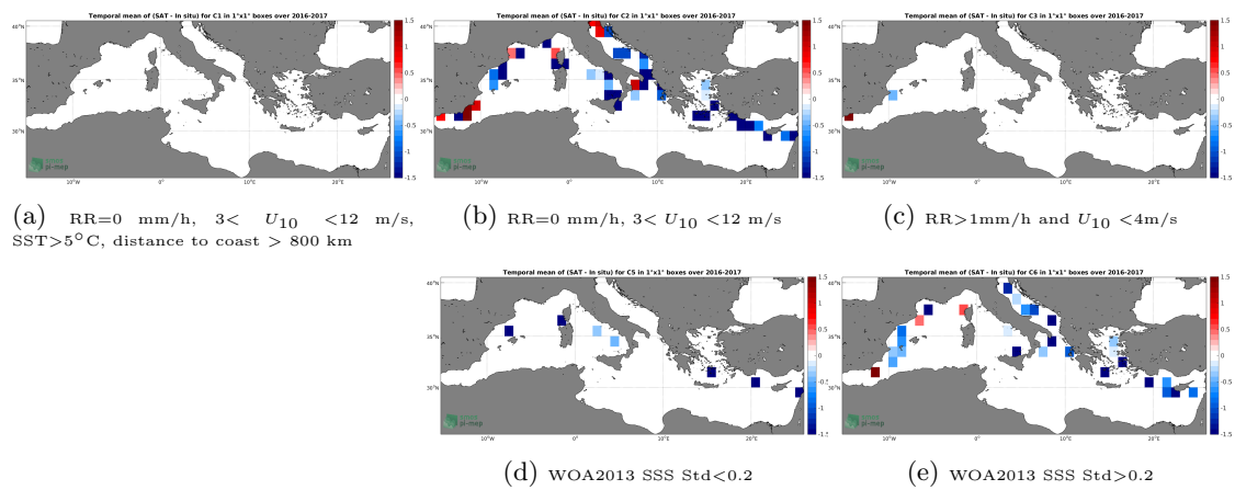
Figure 12: Temporal mean gridded over spatial boxes of size 1^\circ \times 1^\circ of \Delta SSS (SMAP-L2-JPL-V4.3 - TSG-GOSUD-Sailing-ship) for 5 different subdatasets corresponding to:RR=0 mm/h, 3 < U_{10} < 12 m/s, SST>5°C, distance to coast > 800 km (a), RR=0 mm/h, 3 < U_{10} < 12 m/s (b), RR>1mm/h and U_{10} < 4 m/s (c), WOA2013 SSS Std<0.2 (d), WOA2013 SSS Std>0.2 (e).
