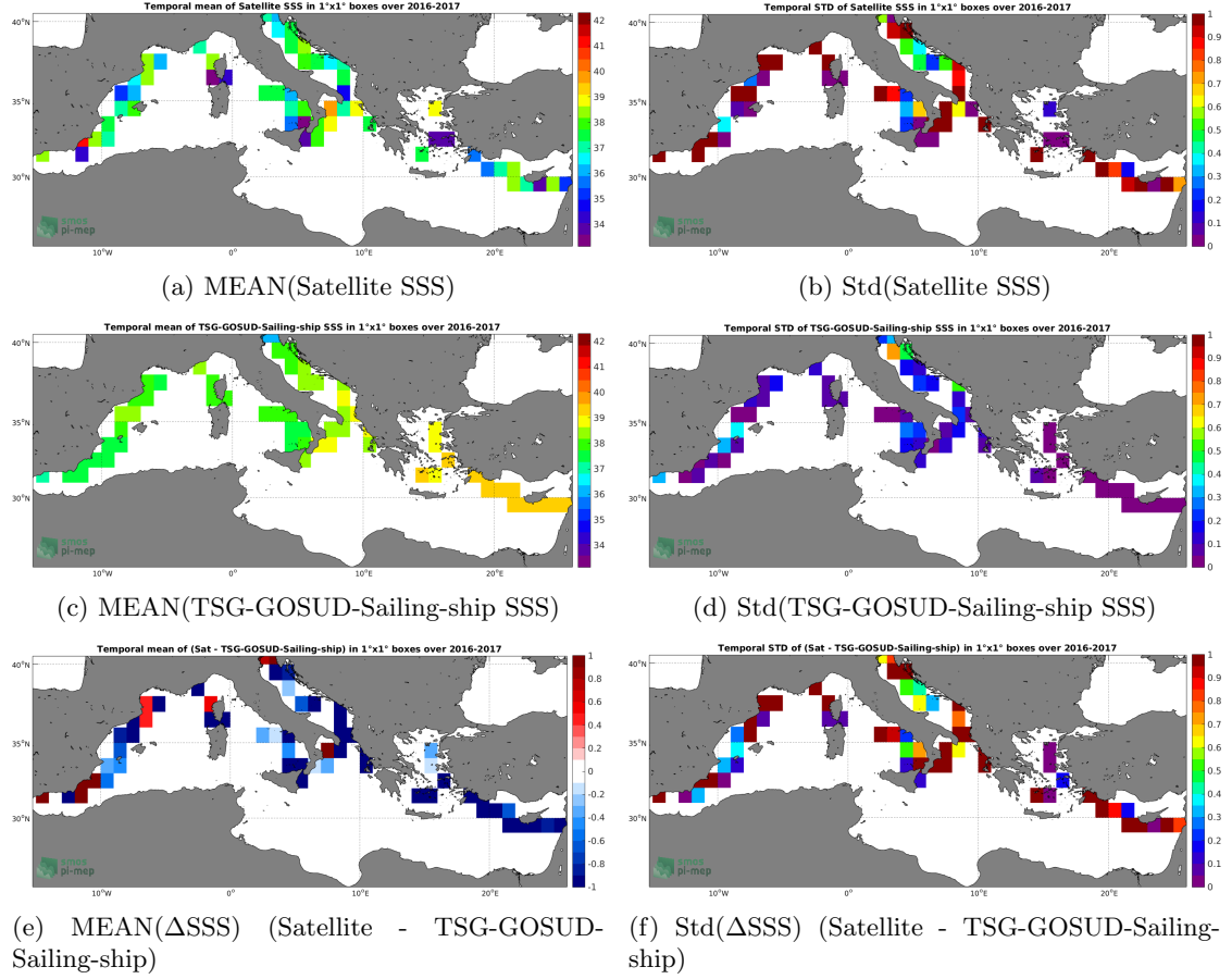
Figure 6: Temporal mean (left) and Std (right) of SSS from SMAP-L2-JPL-V4.3 (top), TSG-GOSUD-Sailing-ship (middle), and of \Delta SSS (Satellite - TSG-GOSUD-Sailing-ship). Only match-up pairs are used to generate these maps.
