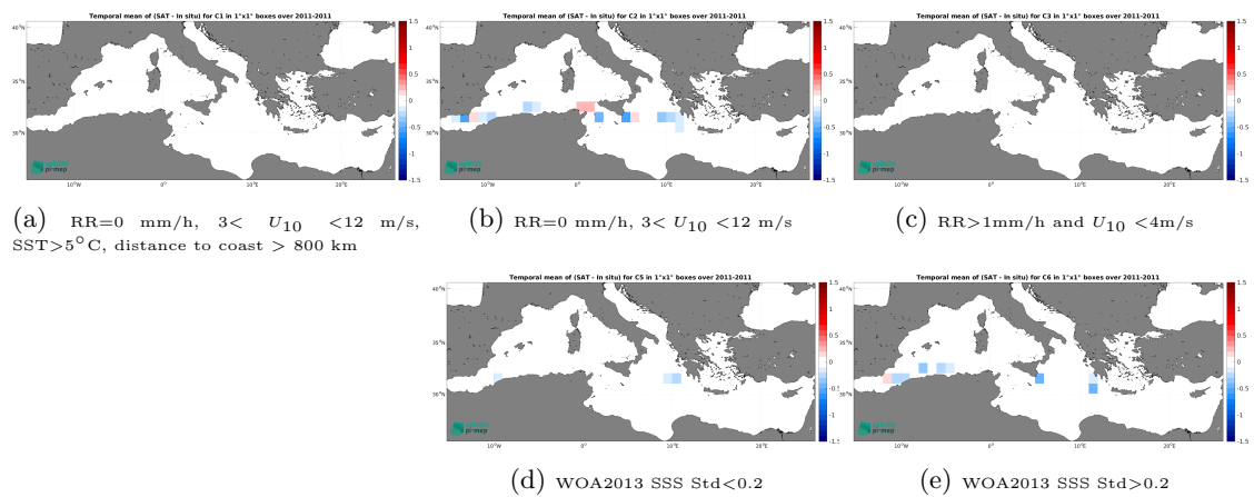
Figure 14: Temporal mean gridded over spatial boxes of size 1^\circ \times 1^\circ of \Delta SSS (CCI SSS L4 Merged-OI v5.5 - 7-day running (ESA) - TSG (SAMOS)) for 5 different subdatasets corresponding to:RR=0 mm/h, 3 < U_{10} < 12 m/s, SST >5^\circ\text{C} , distance to coast > 800 km (a), RR=0 mm/h, 3 < U_{10} < 12 m/s (b), RR >1 mm/h and U_{10} < 4 m/s (c), WOA2013 SSS Std <0.2 (d), WOA2013 SSS Std >0.2 (e).
