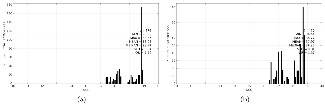
Figure 3: Histograms of SSS from TSG (SAMOS) (a) and CCI SSS L4 Merged-OI v5.5 - 7-day running (ESA) (b) considering all match-up pairs per bins of 0.1 over the Mediterranean Sea Pi-MEP region and for the full satellite product period.
