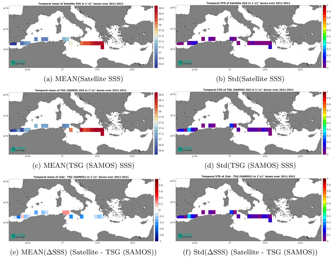
Figure 7: Temporal mean (left) and Std (right) of SSS from CCI SSS L4 Merged-OI v5.5 - 7-day running (ESA) (top), TSG (SAMOS) (middle), and of \Delta SSS (Satellite - TSG (SAMOS)). Only match-up pairs are used to generate these maps.
