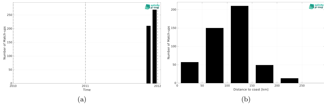
Figure 2: Number of match-ups between TSG (SAMOS) and CCI SSS L4 Merged-OI v5.5 - 7-day running (ESA) SSS as a function of time (a) and as function of the distance to coast (b) over the Mediterranean Sea Pi-MEP region and for the full satellite product period.
