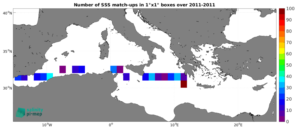
Figure 5: Number of SSS match-ups between TSG (SAMOS) SSS and the CCI SSS L4 Merged-OI v5.5 - 7-day running (ESA) SSS product for the Mediterranean Sea Pi-MEP region over 1^\circ \times 1^\circ boxes and for the full satellite product period.
