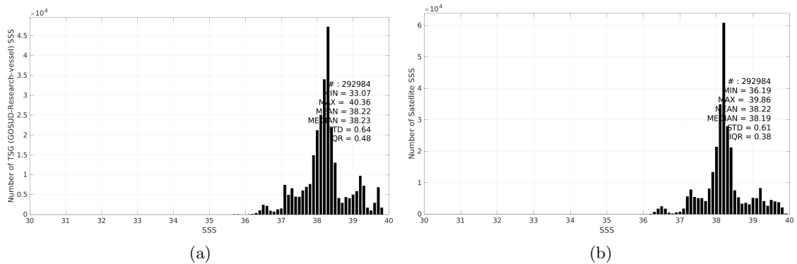
Figure 3: Histograms of SSS from TSG (GOSUD-Research-vessel) (a) and CCI SSS L4 Merged-OI v5.5 - 7-day running (ESA) (b) considering all match-up pairs per bins of 0.1 over the Mediterranean Sea Pi-MEP region and for the full satellite product period.
