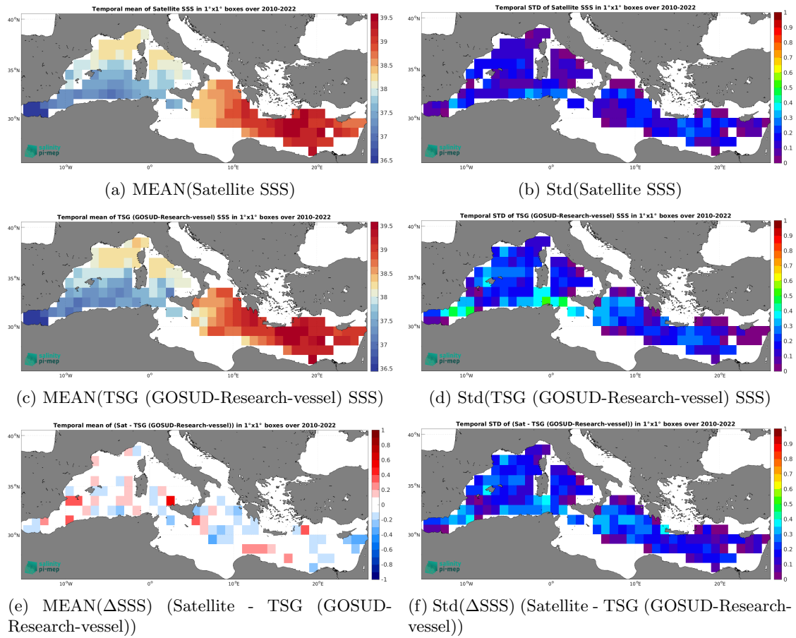
Figure 7: Temporal mean (left) and Std (right) of SSS from CCI SSS L4 Merged-OI v5.5 - 7-day running (ESA) (top), TSG (GOSUD-Research-vessel) (middle), and of \Delta SSS (Satellite - TSG (GOSUD-Research-vessel)). Only match-up pairs are used to generate these maps.
