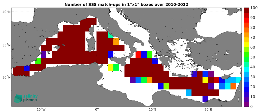
Figure 5: Number of SSS match-ups between TSG (GOSUD-Research-vessel) SSS and the CCI SSS L4 Merged-OI v5.5 - 7-day running (ESA) SSS product for the Mediterranean Sea Pi-MEP region over 1^\circ \times 1^\circ boxes and for the full satellite product period.
