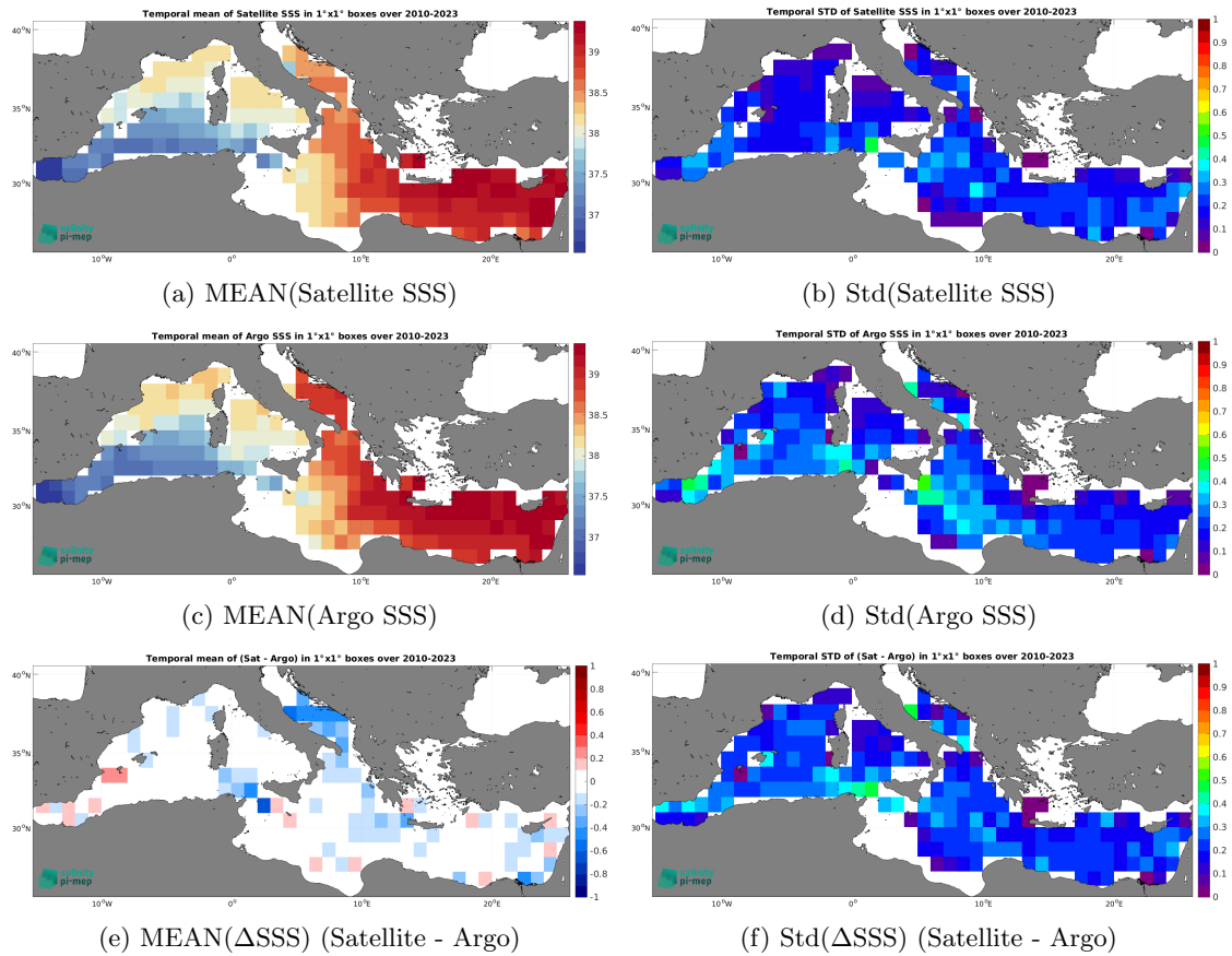
Figure 7: Temporal mean (left) and Std (right) of SSS from CCI SSS L4 Merged-OI v5.5 - 7-day running (ESA) (top), Argo (middle), and of \Delta SSS (Satellite - Argo). Only match-up pairs are used to generate these maps.
