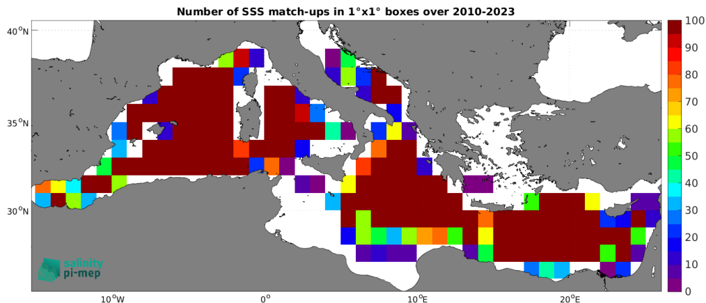
Figure 5: Number of SSS match-ups between Argo SSS and the CCI SSS L4 Merged-OI v5.5 - 7-day running (ESA) SSS product for the Mediterranean Sea Pi-MEP region over 1^\circ \times 1^\circ boxes and for the full satellite product period.
