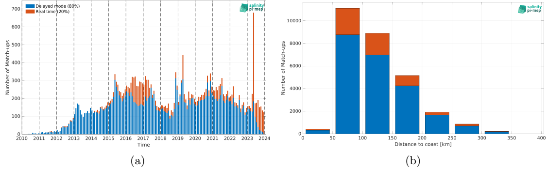
Figure 2: Number of match-ups between Argo and CCI SSS L4 Merged-OI v5.5 - 7-day running (ESA) SSS as a function of time (a) and as function of the distance to coast (b) over the Mediterranean Sea Pi-MEP region and for the full satellite product period.
