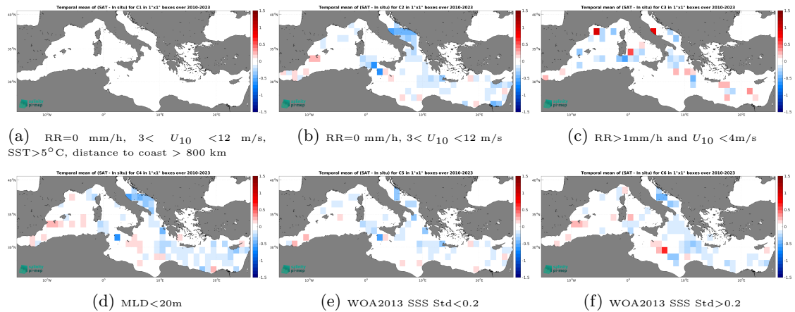
Figure 14: Temporal mean gridded over spatial boxes of size 1^\circ \times 1^\circ of \Delta SSS (CCI SSS L4 Merged-OI v5.5 - 7-day running (ESA) - Argo) for 6 different subdatasets corresponding to:RR=0 mm/h, 3 < U_{10} < 12 m/s, SST >5^\circ C, distance to coast > 800 km (a), RR=0 mm/h, 3 < U_{10} < 12 m/s (b), RR >1 mm/h and U_{10} < 4 m/s (c),MLD <20 m (d),WOA2013 SSS Std <0.2 (e),WOA2013 SSS Std >0.2 (f).
