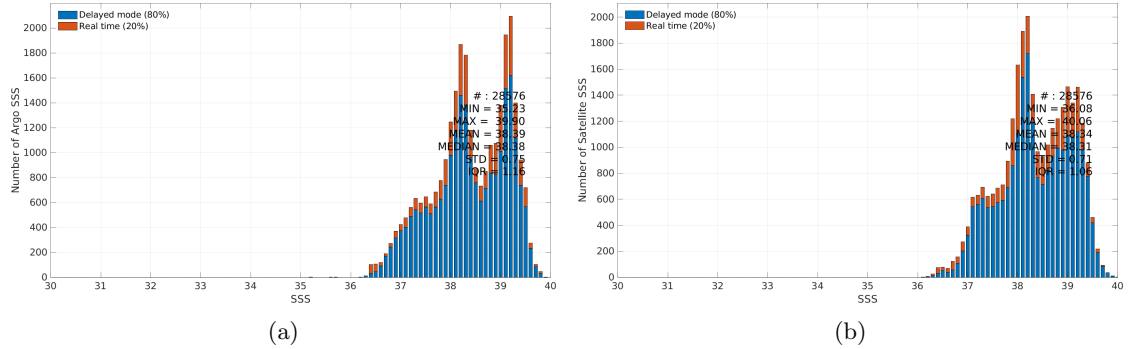
Figure 3: Histograms of SSS from Argo (a) and CCI SSS L4 Merged-OI v5.5 - 7-day running (ESA) (b) considering all match-up pairs per bins of 0.1 over the Mediterranean Sea Pi-MEP region and for the full satellite product period.
