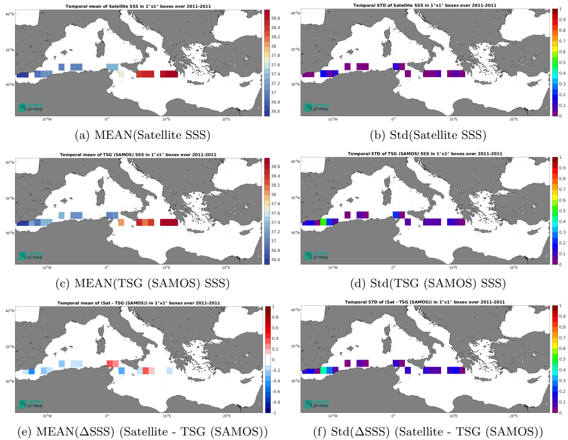
Figure 7: Temporal mean (left) and Std (right) of SSS from CCI SSS L4 Merged-OI v5.5 - 30-day running (ESA) (top), TSG (SAMOS) (middle), and of \Delta SSS (Satellite - TSG (SAMOS)). Only match-up pairs are used to generate these maps.
