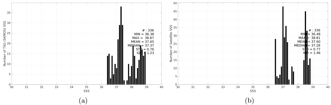
Figure 3: Histograms of SSS from TSG (SAMOS) (a) and CCI SSS L4 Merged-OI v5.5 - 30-day running (ESA) (b) considering all match-up pairs per bins of 0.1 over the Mediterranean Sea Pi-MEP region and for the full satellite product period.
