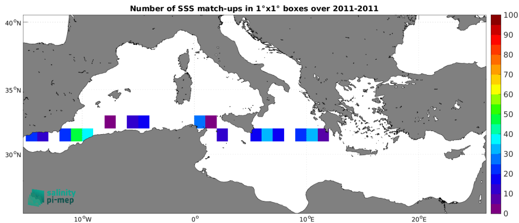
Figure 5: Number of SSS match-ups between TSG (SAMOS) SSS and the CCI SSS L4 Merged-OI v5.5 - 30-day running (ESA) SSS product for the Mediterranean Sea Pi-MEP region over 1^\circ \times 1^\circ boxes and for the full satellite product period.
