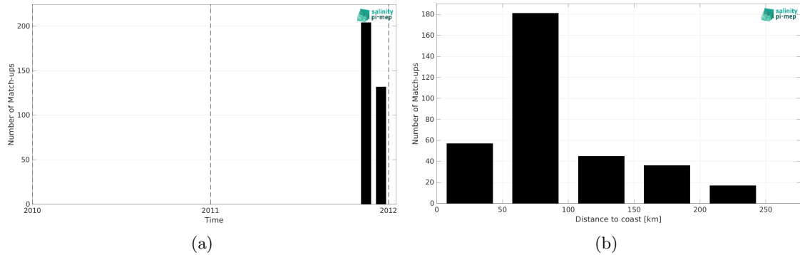
Figure 2: Number of match-ups between TSG (SAMOS) and CCI SSS L4 Merged-OI v5.5 - 30-day running (ESA) SSS as a function of time (a) and as function of the distance to coast (b) over the Mediterranean Sea Pi-MEP region and for the full satellite product period.
