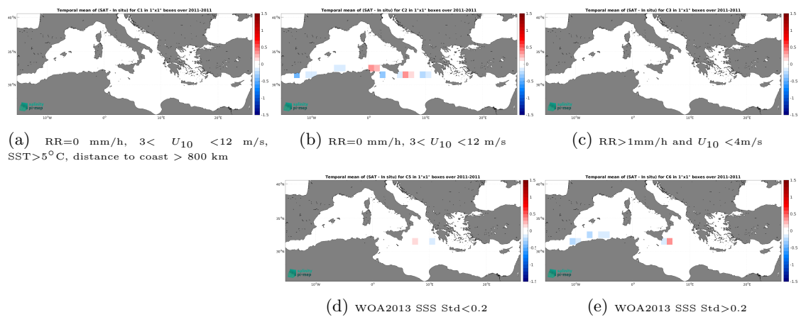
Figure 14: Temporal mean gridded over spatial boxes of size 1^\circ \times 1^\circ of \Delta\text{SSS} (CCI SSS L4 Merged-OI v5.5 - 30-day running (ESA) - TSG (SAMOS)) for 5 different subdatasets corresponding to:RR=0 mm/h, 3 < U_{10} < 12 m/s, SST>5°C, distance to coast > 800 km (a), RR=0 mm/h, 3 < U_{10} < 12 m/s (b), RR>1mm/h and U_{10} < 4 m/s (c), WOA2013 SSS Std<0.2 (d), WOA2013 SSS Std>0.2 (e).
