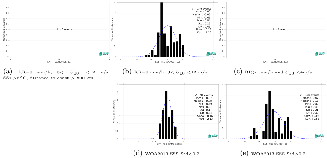
Figure 15: Normalized histogram of \Delta SSS (CCI SSS L4 Merged-OI v5.5 - 30-day running (ESA) - TSG (SAMOS)) for 5 different subdatasets corresponding to: RR=0 mm/h, 3 < U_{10} < 12 m/s, SST > 5°C, distance to coast > 800 km (a), RR=0 mm/h, 3 < U_{10} < 12 m/s (b), RR > 1mm/h and U_{10} < 4 m/s (c), WOA2013 SSS Std < 0.2 (d), WOA2013 SSS Std > 0.2 (e).
