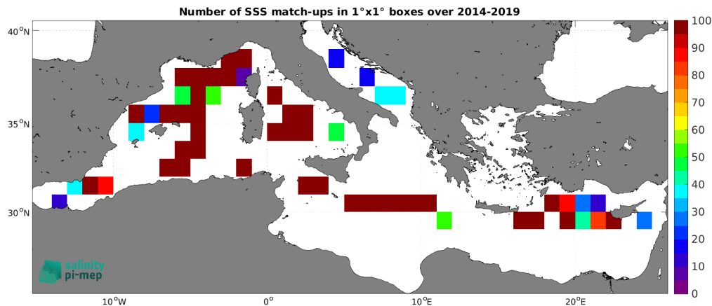
Figure 5: Number of SSS match-ups between TSG (GOSUD-Sailing-ship) SSS and the CCI SSS L4 Merged-OI v5.5 - 30-day running (ESA) SSS product for the Mediterranean Sea Pi-MEP region over 1^\circ \times 1^\circ boxes and for the full satellite product period.
