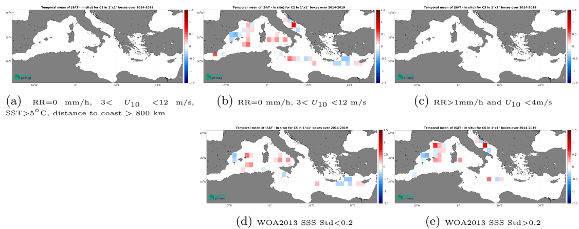
Figure 14: Temporal mean gridded over spatial boxes of size 1^\circ \times 1^\circ of \Delta SSS (CCI SSS L4 Merged-OI v5.5 - 30-day running (ESA) - TSG (GOSUD-Sailing-ship)) for 5 different subdatasets corresponding to:RR=0 mm/h, 3 < U_{10} < 12 m/s, SST >5^\circ C, distance to coast > 800 km (a), RR=0 mm/h, 3 < U_{10} < 12 m/s (b), RR >1 mm/h and U_{10} < 4 m/s (c), WOA2013 SSS Std <0.2 (d), WOA2013 SSS Std >0.2 (e).
