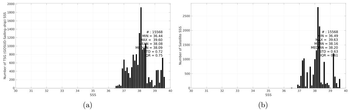
Figure 3: Histograms of SSS from TSG (GOSUD-Sailing-ship) (a) and CCI SSS L4 Merged-OI v5.5 - 30-day running (ESA) (b) considering all match-up pairs per bins of 0.1 over the Mediterranean Sea Pi-MEP region and for the full satellite product period.
