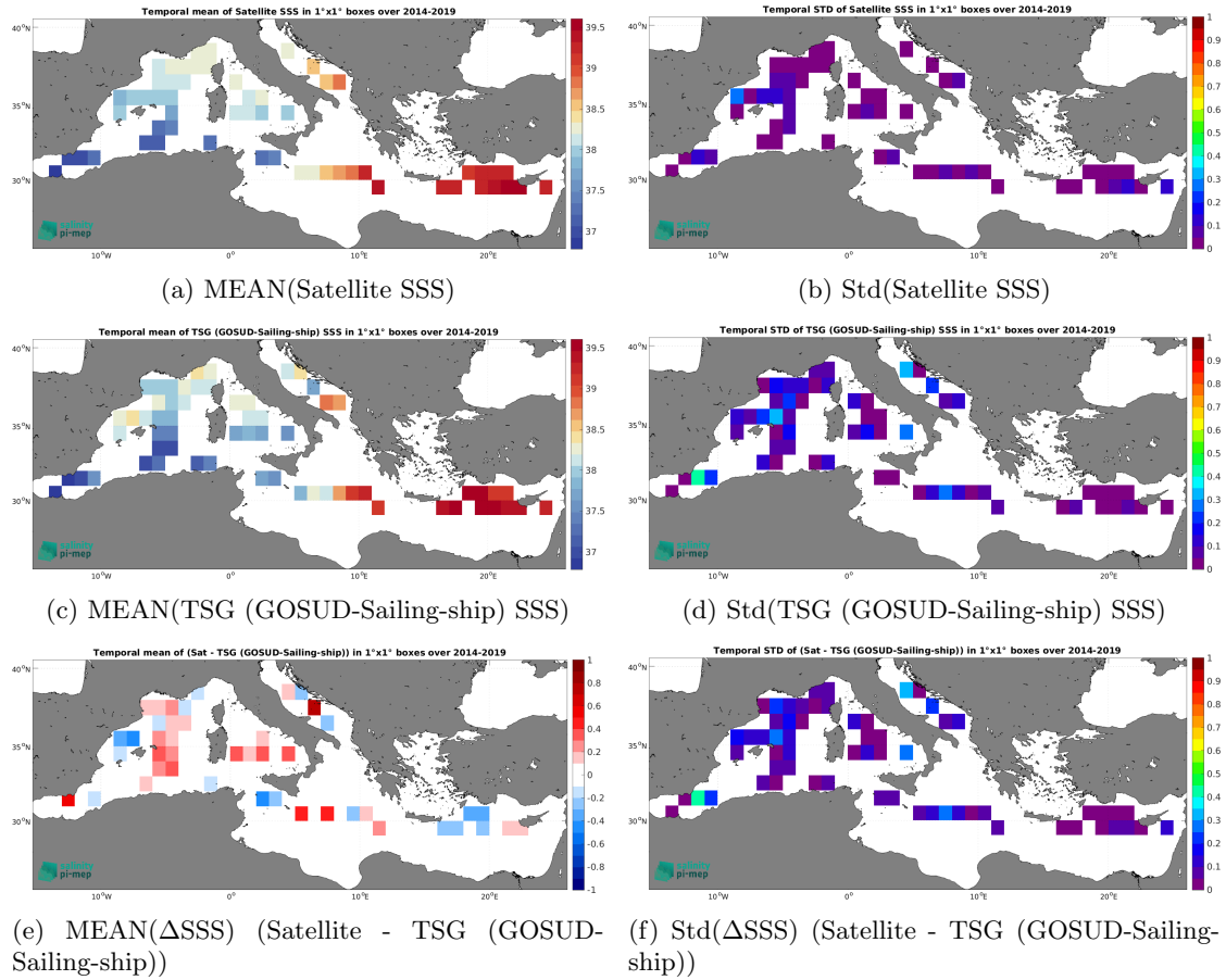
Figure 7: Temporal mean (left) and Std (right) of SSS from CCI SSS L4 Merged-OI v5.5 - 30-day running (ESA) (top), TSG (GOSUD-Sailing-ship) (middle), and of \Delta SSS (Satellite - TSG (GOSUD-Sailing-ship)). Only match-up pairs are used to generate these maps.
