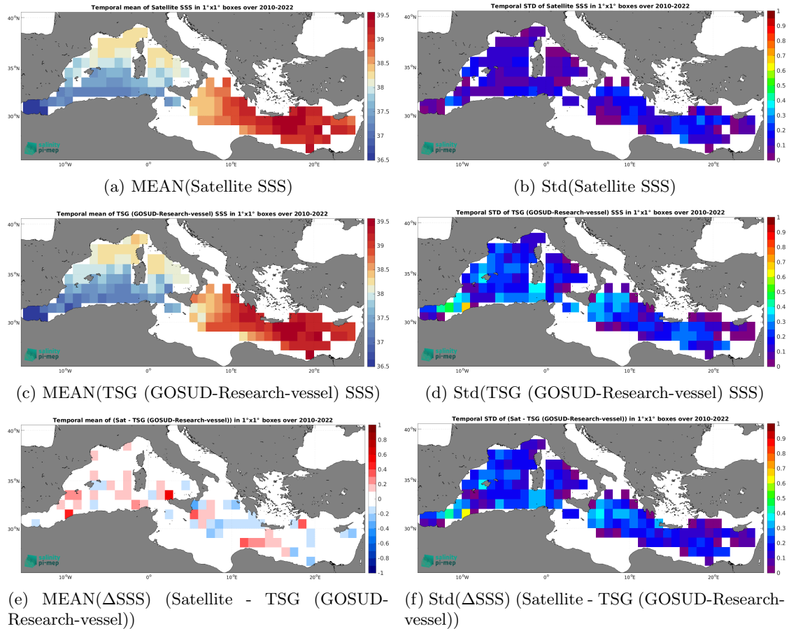
Figure 7: Temporal mean (left) and Std (right) of SSS from CCI SSS L4 Merged-OI v5.5 - 30-day running (ESA) (top), TSG (GOSUD-Research-vessel) (middle), and of \Delta SSS (Satellite - TSG (GOSUD-Research-vessel)). Only match-up pairs are used to generate these maps.
