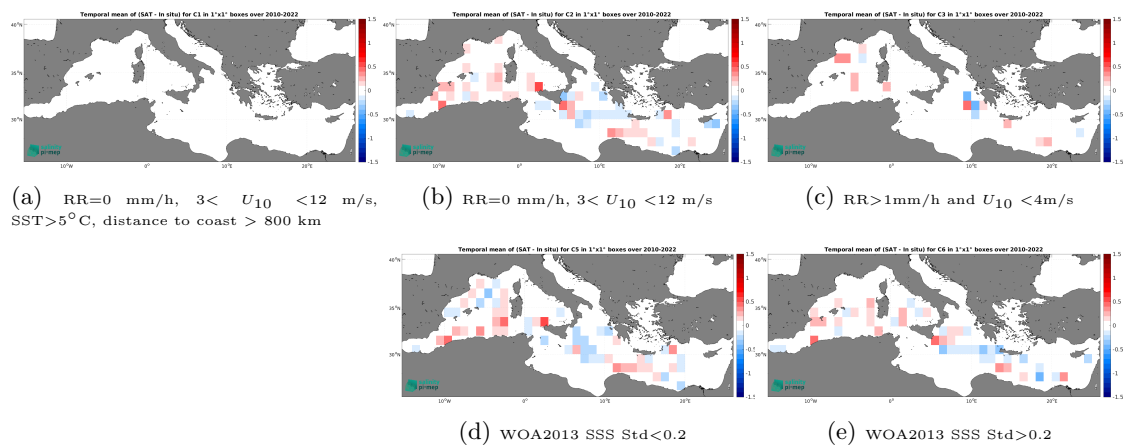
Figure 14: Temporal mean gridded over spatial boxes of size 1^\circ \times 1^\circ of \Delta\text{SSS} (CCI SSS L4 Merged-OI v5.5 - 30-day running (ESA) - TSG (GOSUD-Research-vessel)) for 5 different subdatasets corresponding to:RR=0 mm/h, 3 < U_{10} < 12 m/s, SST >5^\circ\text{C} , distance to coast > 800 km (a), RR=0 mm/h, 3 < U_{10} < 12 m/s (b), RR >1 mm/h and U_{10} < 4 m/s (c), WOA2013 SSS Std <0.2 (d), WOA2013 SSS Std >0.2 (e).
