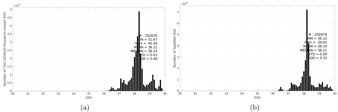
Figure 3: Histograms of SSS from TSG (GOSUD-Research-vessel) (a) and CCI SSS L4 Merged-OI v5.5 - 30-day running (ESA) (b) considering all match-up pairs per bins of 0.1 over the Mediterranean Sea Pi-MEP region and for the full satellite product period.
