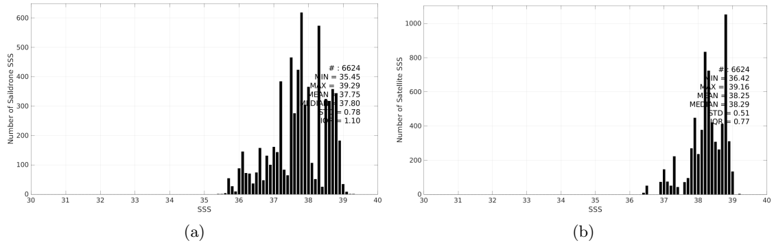
Figure 3: Histograms of SSS from Saildrone (a) and CCI SSS L4 Merged-OI v5.5 - 30-day running (ESA) (b) considering all match-up pairs per bins of 0.1 over the Mediterranean Sea Pi-MEP region and for the full satellite product period.
