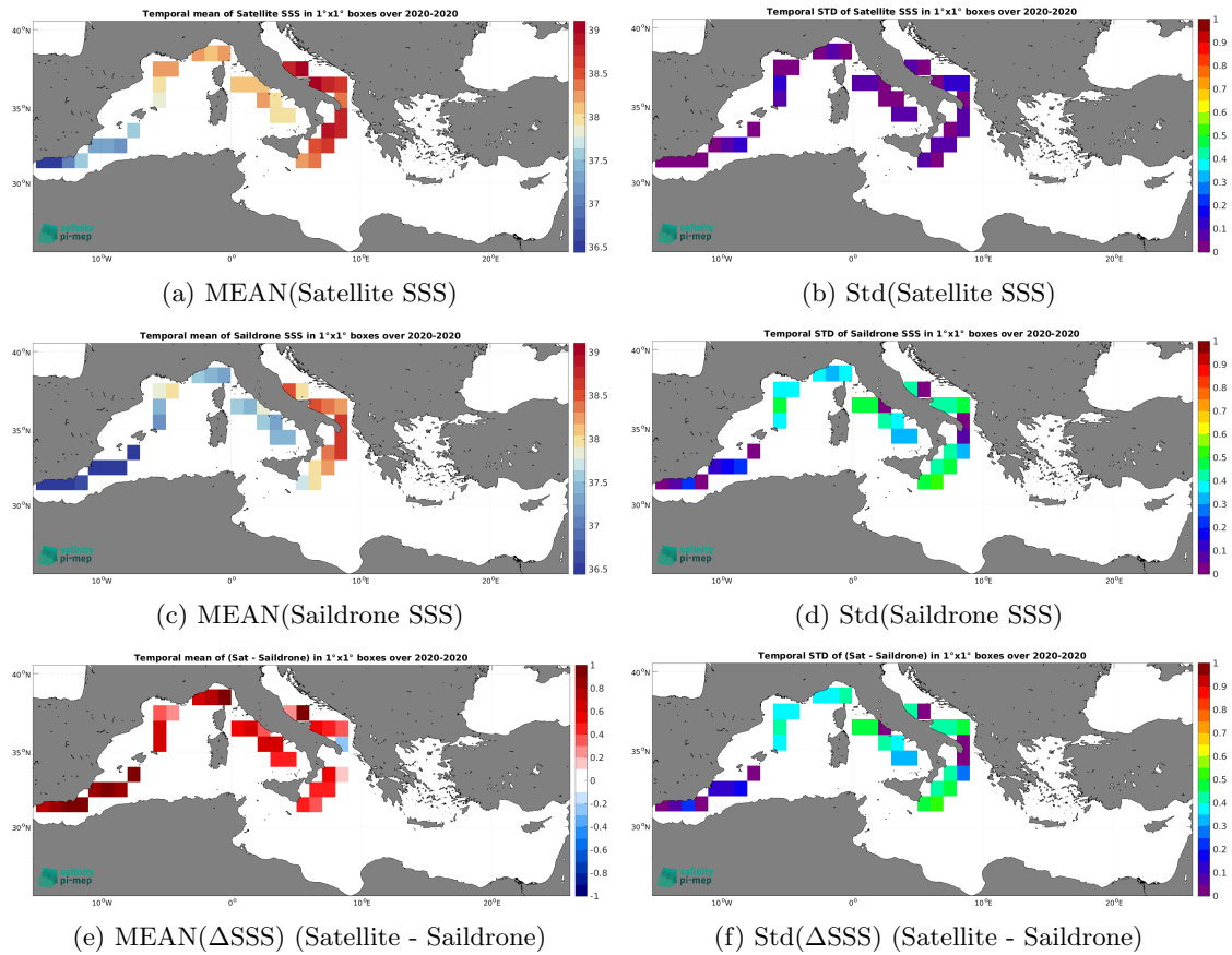
Figure 7: Temporal mean (left) and Std (right) of SSS from CCI SSS L4 Merged-OI v5.5 - 30-day running (ESA) (top), Saildrone (middle), and of \Delta SSS (Satellite - Saildrone). Only match-up pairs are used to generate these maps.
