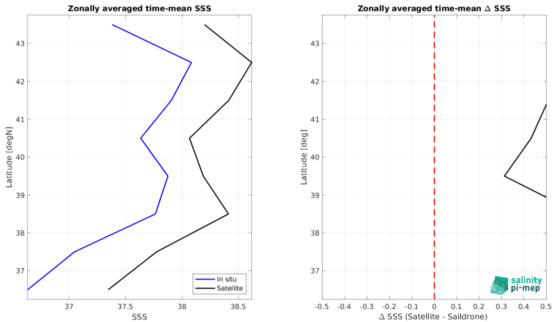
Figure 9: Left panel: Zonal mean SSS from CCI SSS L4 Merged-OI v5.5 - 30-day running (ESA) satellite product (black) and from Sairdron (blue). Right panel: Zonal mean of \Delta SSS (Satellite - Sairdron) for all the collected Pi-MEP match-up pairs estimated over the full satellite product period.
