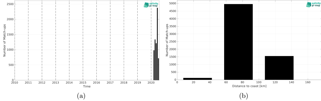
Figure 2: Number of match-ups between Saildrone and CCI SSS L4 Merged-OI v5.5 - 30-day running (ESA) SSS as a function of time (a) and as function of the distance to coast (b) over the Mediterranean Sea Pi-MEP region and for the full satellite product period.
