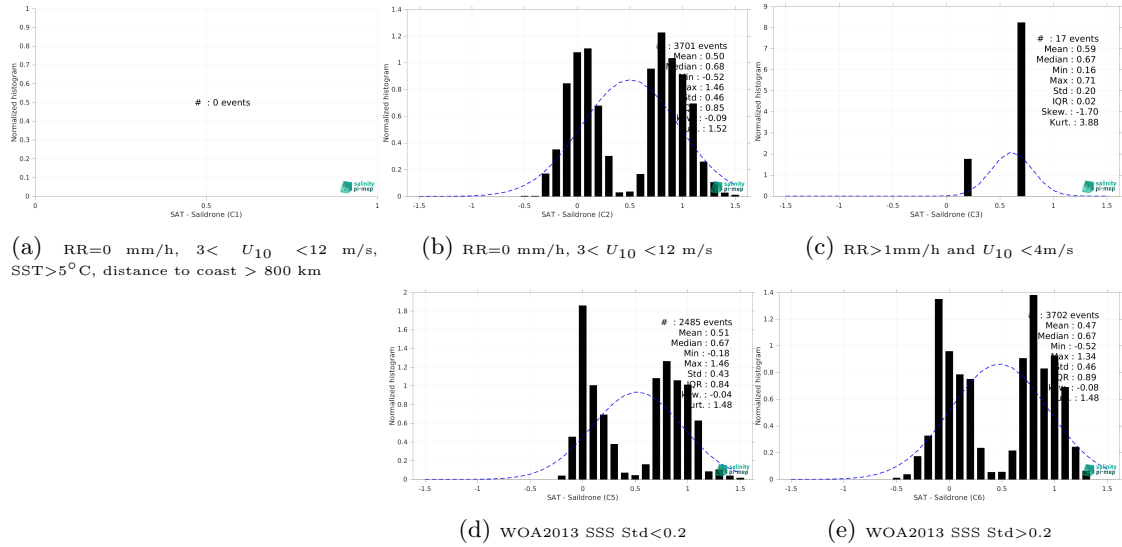
Figure 15: Normalized histogram of \Delta\text{SSS} (CCI SSS L4 Merged-OI v5.5 - 30-day running (ESA) - Saldrone) for 5 different subdatasets corresponding to: RR=0 mm/h, 3 < U_{10} < 12 m/s, SST > 5^{\circ}\text{C} , distance to coast > 800 km (a), RR=0 mm/h, 3 < U_{10} < 12 m/s (b), RR > 1\text{mm/h} and U_{10} < 4\text{m/s} (c), WOA2013 SSS Std < 0.2 (d), WOA2013 SSS Std > 0.2 (e).
