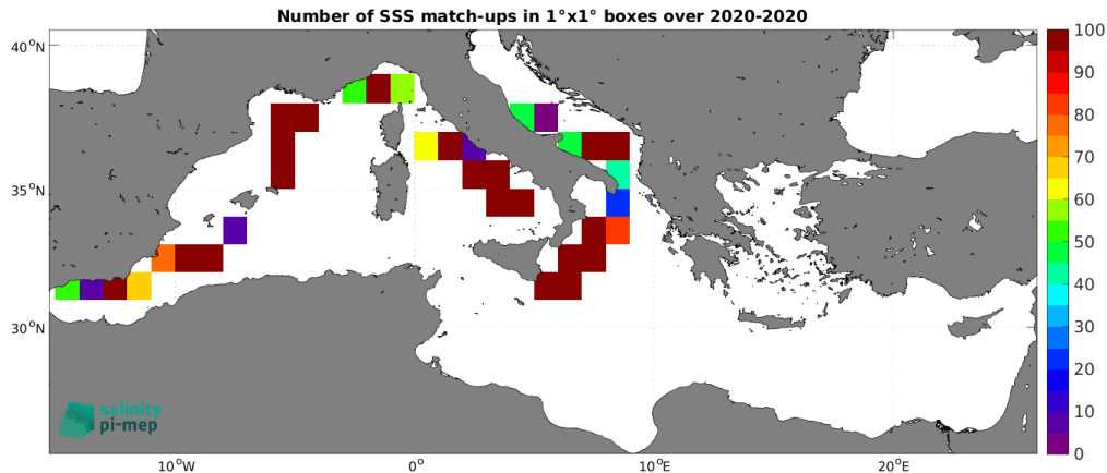
Figure 5: Number of SSS match-ups between Saildrone SSS and the CCI SSS L4 Merged-OI v5.5 - 30-day running (ESA) SSS product for the Mediterranean Sea Pi-MEP region over 1^\circ \times 1^\circ boxes and for the full satellite product period.
