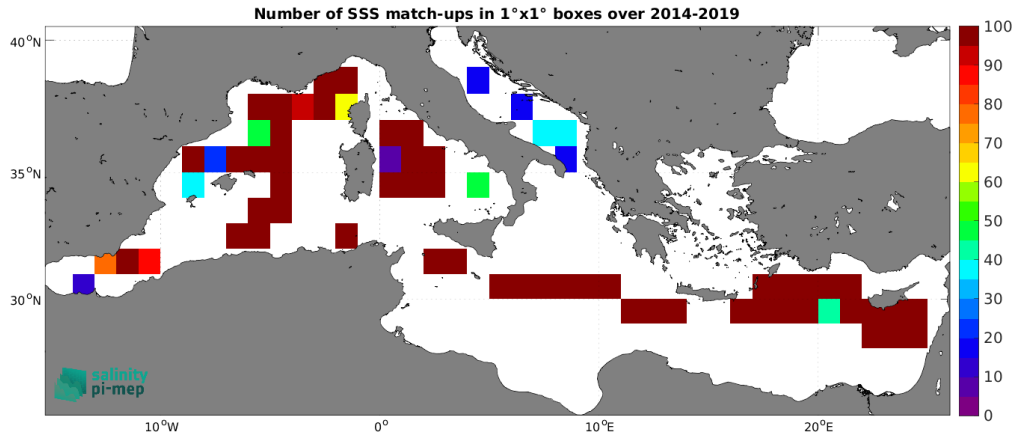
Figure 5: Number of SSS match-ups between TSG (GOSUD-Sailing-ship) SSS and the CCI SSS L4 Merged-OI v4.41 - 7-day running (ESA) SSS product for the Mediterranean Sea Pi-MEP region over 1^\circ \times 1^\circ boxes and for the full satellite product period.
