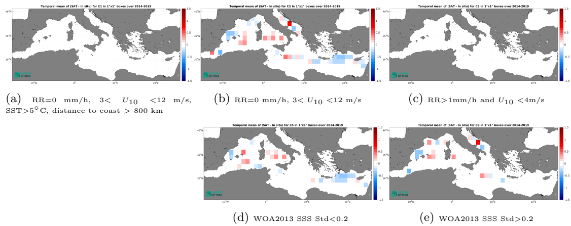
Figure 14: Temporal mean gridded over spatial boxes of size 1^\circ \times 1^\circ of \Delta SSS (CCI SSS L4 Merged-OI v4.41 - 7-day running (ESA) - TSG (GOSUD-Sailing-ship)) for 5 different subdatasets corresponding to:RR=0 mm/h, 3 < U_{10} < 12 m/s, SST >5^\circ\text{C} , distance to coast > 800 km (a), RR=0 mm/h, 3 < U_{10} < 12 m/s (b), RR >1 mm/h and U_{10} < 4 m/s (c), WOA2013 SSS Std <0.2 (d), WOA2013 SSS Std >0.2 (e).
