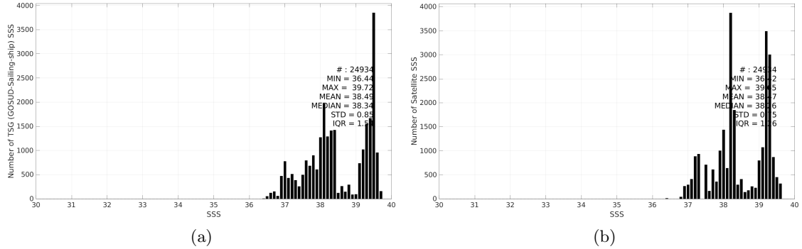
Figure 3: Histograms of SSS from TSG (GOSUD-Sailing-ship) (a) and CCI SSS L4 Merged-OI v4.41 - 7-day running (ESA) (b) considering all match-up pairs per bins of 0.1 over the Mediterranean Sea Pi-MEP region and for the full satellite product period.
