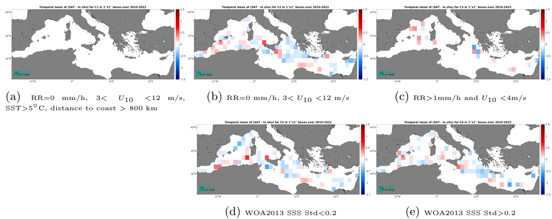
Figure 14: Temporal mean gridded over spatial boxes of size 1^\circ \times 1^\circ of \Delta\text{SSS} (CCI SSS L4 Merged-OI v4.41 - 7-day running (ESA) - TSG (GOSUD-Research-vessel)) for 5 different subdatasets corresponding to:RR=0 mm/h, 3 < U_{10} < 12 m/s, SST>5°C, distance to coast > 800 km (a), RR=0 mm/h, 3 < U_{10} < 12 m/s (b), RR>1mm/h and U_{10} < 4 m/s (c), WOA2013 SSS Std<0.2 (d), WOA2013 SSS Std>0.2 (e).
