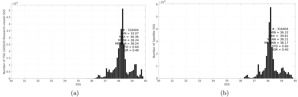
Figure 3: Histograms of SSS from TSG (GOSUD-Research-vessel) (a) and CCI SSS L4 Merged-OI v4.41 - 7-day running (ESA) (b) considering all match-up pairs per bins of 0.1 over the Mediterranean Sea Pi-MEP region and for the full satellite product period.
