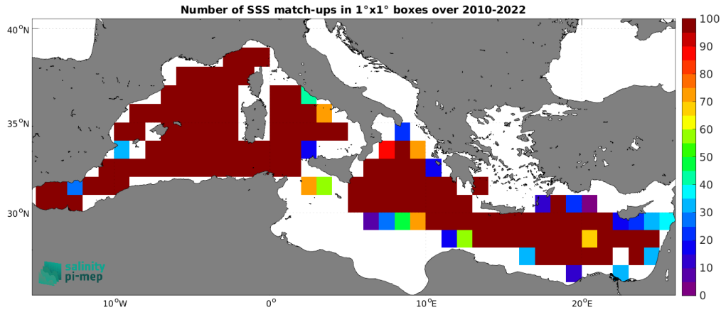
Figure 5: Number of SSS match-ups between TSG (GOSUD-Research-vessel) SSS and the CCI SSS L4 Merged-OI v4.41 - 7-day running (ESA) SSS product for the Mediterranean Sea Pi-MEP region over 1^\circ \times 1^\circ boxes and for the full satellite product period.
