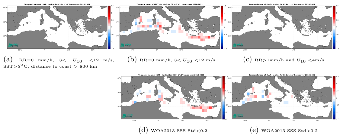
Figure 14: Temporal mean gridded over spatial boxes of size 1^\circ \times 1^\circ of \Delta\text{SSS} (CCI SSS L4 Merged-OI v4.41 - 7-day running (ESA) - TSG (CSIC-UTM)) for 5 different subdatasets corresponding to: RR=0 mm/h, 3 < U_{10} < 12 m/s, SST > 5°C, distance to coast > 800 km (a), RR=0 mm/h, 3 < U_{10} < 12 m/s (b), RR > 1 mm/h and U_{10} < 4 m/s (c), WOA2013 SSS Std < 0.2 (d), WOA2013 SSS Std > 0.2 (e).
