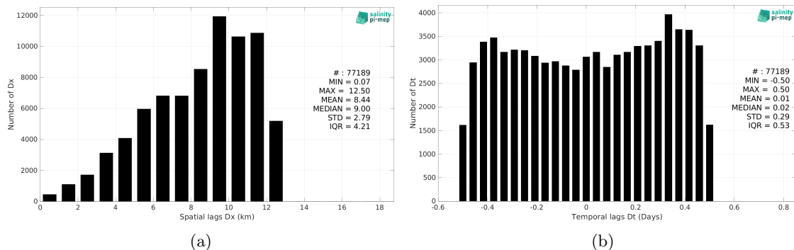
Figure 6: Histograms of the spatial (a) and temporal (b) lags between the location/time of the TSG (CSIC-UTM) measurement and the date of the corresponding CCI SSS L4 Merged-OI v4.41 - 7-day running (ESA) SSS pixel.
