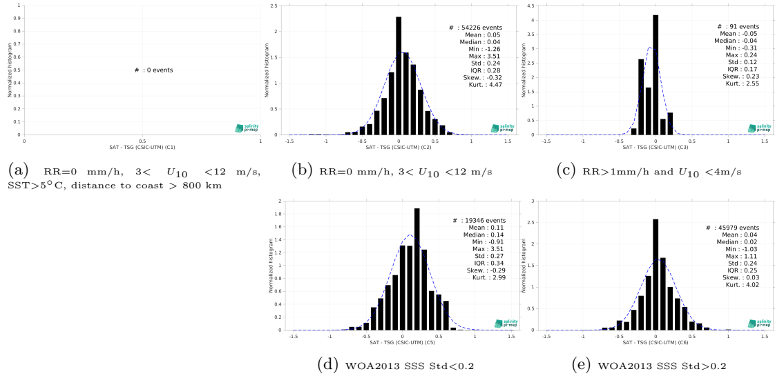
Figure 15: Normalized histogram of \Delta SSS (CCI SSS L4 Merged-OI v4.41 - 7-day running (ESA) - TSG (CSIC-UTM)) for 5 different subdatasets corresponding to: RR=0 mm/h, 3 < U_{10} < 12 m/s, SST > 5°C, distance to coast > 800 km (a), RR=0 mm/h, 3 < U_{10} < 12 m/s (b), RR > 1mm/h and U_{10} < 4 m/s (c), WOA2013 SSS Std < 0.2 (d), WOA2013 SSS Std > 0.2 (e).
