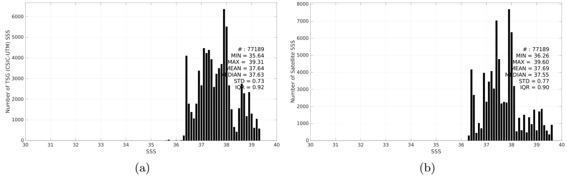
Figure 3: Histograms of SSS from TSG (CSIC-UTM) (a) and CCI SSS L4 Merged-OI v4.41 - 7-day running (ESA) (b) considering all match-up pairs per bins of 0.1 over the Mediterranean Sea Pi-MEP region and for the full satellite product period.
