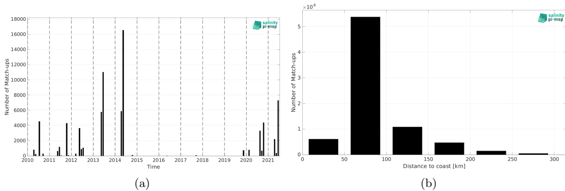
Figure 2: Number of match-ups between TSG (CSIC-UTM) and CCI SSS L4 Merged-OI v4.41 - 7-day running (ESA) SSS as a function of time (a) and as function of the distance to coast (b) over the Mediterranean Sea Pi-MEP region and for the full satellite product period.
