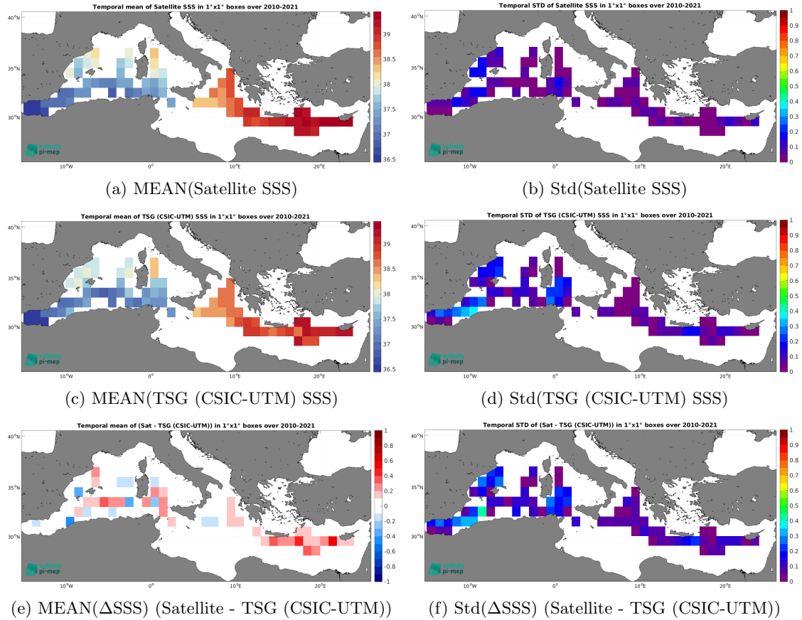
Figure 7: Temporal mean (left) and Std (right) of SSS from CCI SSS L4 Merged-OI v4.41 - 7-day running (ESA) (top), TSG (CSIC-UTM) (middle), and of \Delta\text{SSS} (Satellite - TSG (CSIC-UTM)). Only match-up pairs are used to generate these maps.
