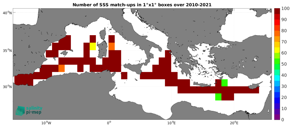
Figure 5: Number of SSS match-ups between TSG (CSIC-UTM) SSS and the CCI SSS L4 Merged-OI v4.41 - 7-day running (ESA) SSS product for the Mediterranean Sea Pi-MEP region over 1^\circ \times 1^\circ boxes and for the full satellite product period.
