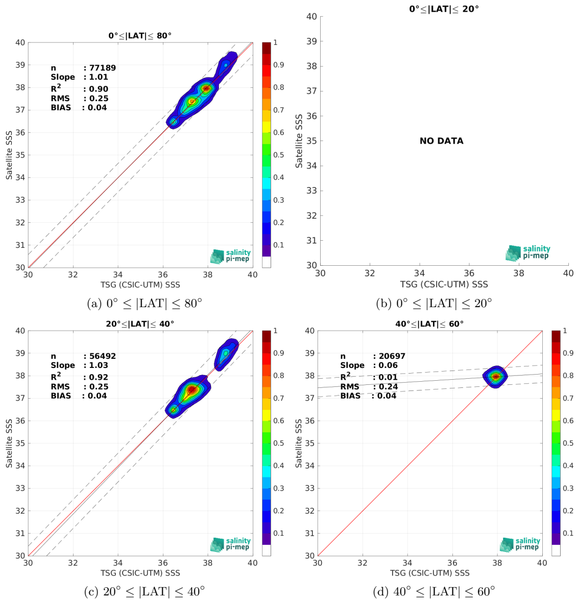
Figure 10: Contour maps of the concentration of CCI SSS L4 Merged-OI v4.41 - 7-day running (ESA) SSS (y-axis) versus TSG (CSIC-UTM) SSS (x-axis) at match-up pairs for different latitude bands. For each plot, the red line shows x=y . The black thin and dashed lines indicate a linear fit through the data cloud and the \pm 95\% confidence levels, respectively. The number match-up pairs n , the slope and R^2 coefficient of the linear fit, the root mean square (RMS) and the mean bias between satellite and in situ data are indicated for each latitude band in each plots.
