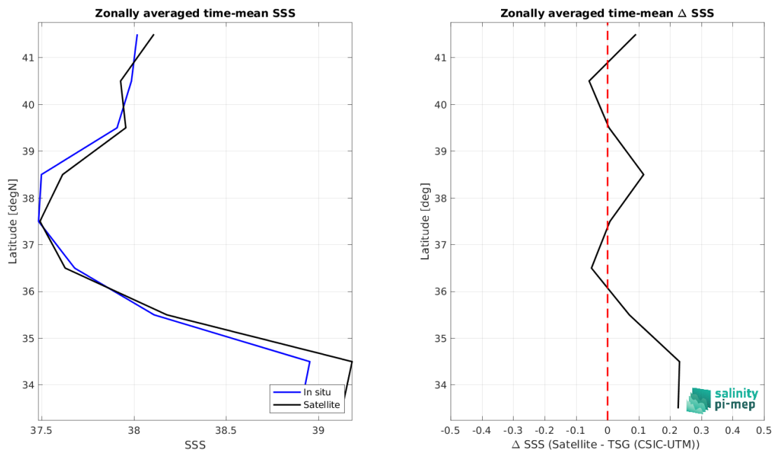
Figure 9: Left panel: Zonal mean SSS from CCI SSS L4 Merged-OI v4.41 - 7-day running (ESA) satellite product (black) and from TSG (CSIC-UTM) (blue). Right panel: Zonal mean of \Delta SSS (Satellite - TSG (CSIC-UTM)) for all the collected Pi-MEP match-up pairs estimated over the full satellite product period.
