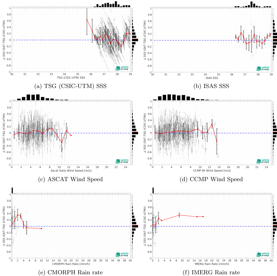
Figure 12: \Delta\text{SSS} (Satellite - TSG (CSIC-UTM)) sorted as function of TSG (CSIC-UTM) SSS values (a), ISAS SSS (b), ASCAT Wind speed (c), CCMP Wind speed (d), CMORPH rain rate (e) and IMERG rain rate (f). In all plots the median and Std of \Delta\text{SSS} for each bin is indicated by the red curves and black vertical thick bars ( \pm 1 Std).
