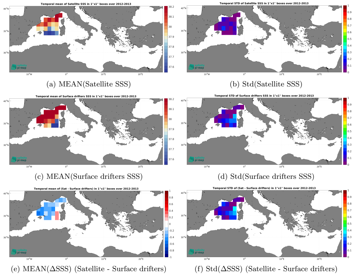
Figure 6: Temporal mean (left) and Std (right) of SSS from CCI SSS L4 Merged-OI v4.41 - 7-day running (ESA) (top), Surface drifters (middle), and of \Delta SSS (Satellite - Surface drifters). Only match-up pairs are used to generate these maps.
