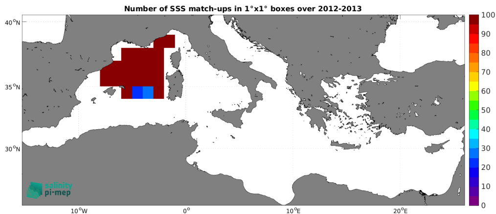
Figure 4: Number of SSS match-ups between Surface drifters SSS and the CCI SSS L4 Merged-OI v4.41 - 7-day running (ESA) SSS product for the Mediterranean Sea Pi-MEP region over 1^\circ \times 1^\circ boxes and for the full satellite product period.
