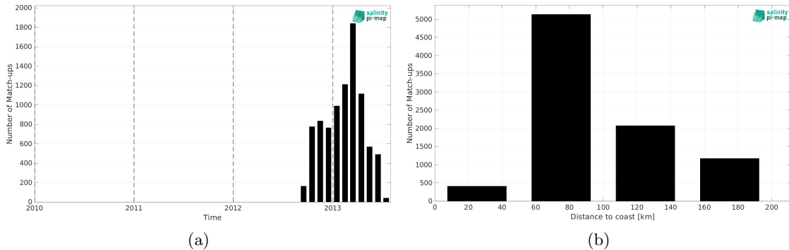
Figure 2: Number of match-ups between Surface drifters and CCI SSS L4 Merged-OI v4.41 - 7-day running (ESA) SSS as a function of time (a) and as function of the distance to coast (b) over the Mediterranean Sea Pi-MEP region and for the full satellite product period.
