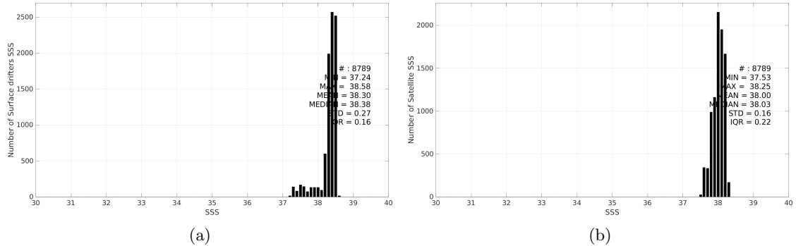
Figure 3: Histograms of SSS from Surface drifters (a) and CCI SSS L4 Merged-OI v4.41 - 7-day running (ESA) (b) considering all match-up pairs per bins of 0.1 over the Mediterranean Sea Pi-MEP region and for the full satellite product period.
