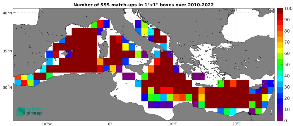
Figure 5: Number of SSS match-ups between Argo SSS and the CCI SSS L4 Merged-OI v4.41 - 7-day running (ESA) SSS product for the Mediterranean Sea Pi-MEP region over 1^\circ \times 1^\circ boxes and for the full satellite product period.
