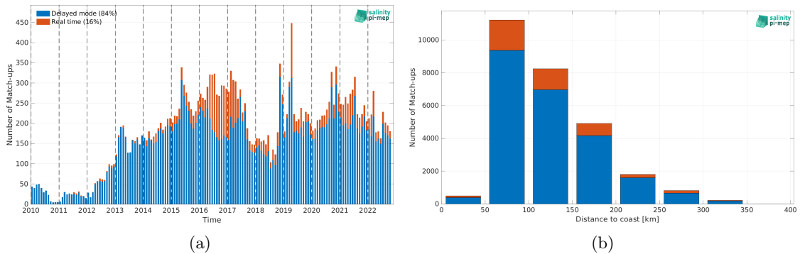
Figure 2: Number of match-ups between Argo and CCI SSS L4 Merged-OI v4.41 - 7-day running (ESA) SSS as a function of time (a) and as function of the distance to coast (b) over the Mediterranean Sea Pi-MEP region and for the full satellite product period.
