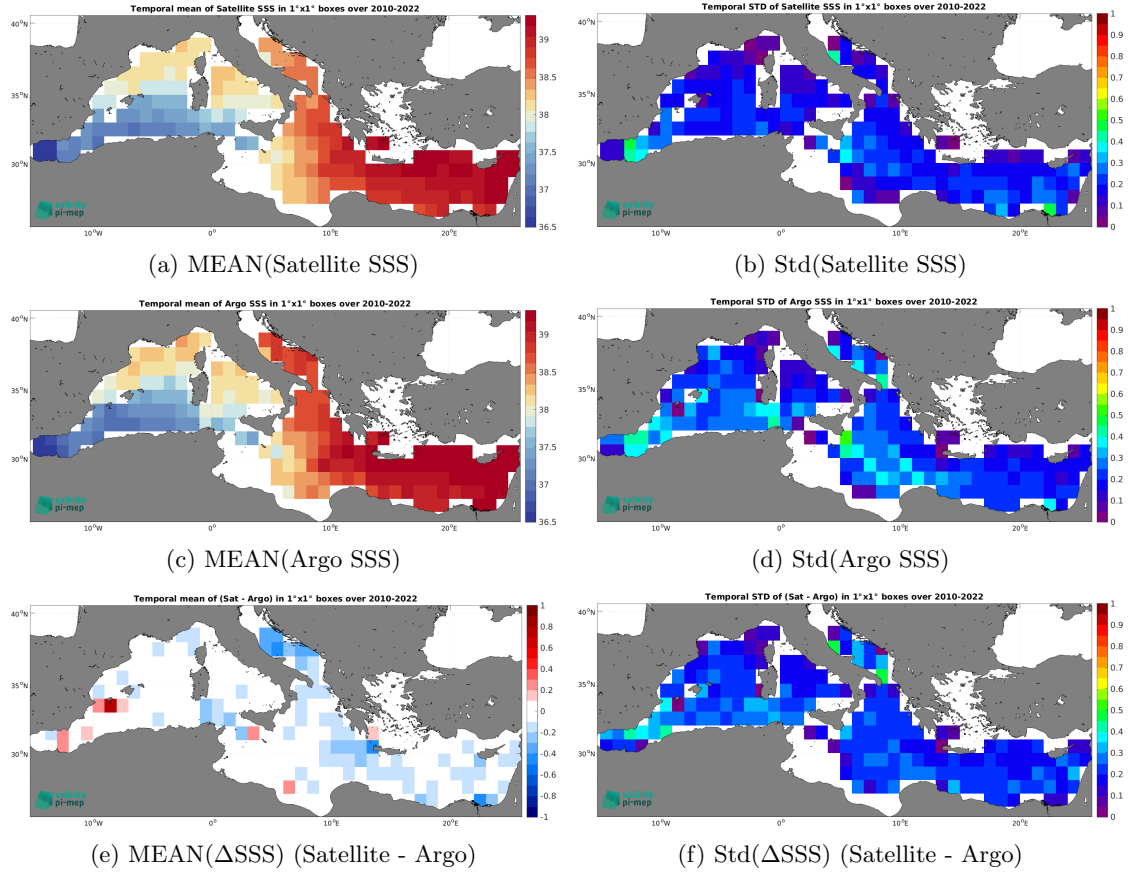
Figure 7: Temporal mean (left) and Std (right) of SSS from CCI SSS L4 Merged-OI v4.41 - 7-day running (ESA) (top), Argo (middle), and of \Delta\text{SSS} (Satellite - Argo). Only match-up pairs are used to generate these maps.
