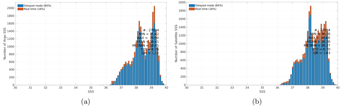
Figure 3: Histograms of SSS from Argo (a) and CCI SSS L4 Merged-OI v4.41 - 7-day running (ESA) (b) considering all match-up pairs per bins of 0.1 over the Mediterranean Sea Pi-MEP region and for the full satellite product period.
