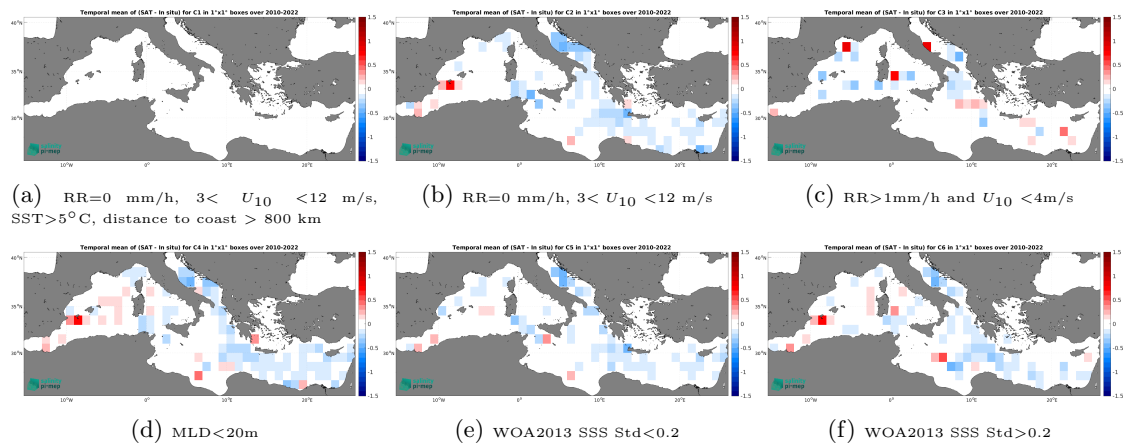
Figure 14: Temporal mean gridded over spatial boxes of size 1^\circ \times 1^\circ of \Delta SSS (CCI SSS L4 Merged-OI v4.41 - 7-day running (ESA) - Argo) for 6 different subdatasets corresponding to:RR=0 mm/h, 3 < U_{10} < 12 m/s, SST >5^\circ C, distance to coast > 800 km (a), RR=0 mm/h, 3 < U_{10} < 12 m/s (b), RR >1 mm/h and U_{10} < 4 m/s (c),MLD <20 m (d),WOA2013 SSS Std <0.2 (e),WOA2013 SSS Std >0.2 (f).
