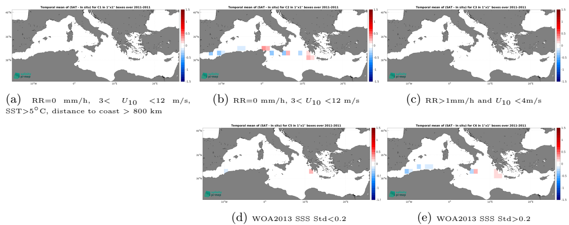
Figure 14: Temporal mean gridded over spatial boxes of size 1^\circ \times 1^\circ of \Delta\text{SSS} (CCI SSS L4 Merged-OI v4.41 - 30-day running (ESA) - TSG (SAMOS)) for 5 different subdatasets corresponding to:RR=0 mm/h, 3 < U_{10} < 12 m/s, SST>5°C, distance to coast > 800 km (a), RR=0 mm/h, 3 < U_{10} < 12 m/s (b), RR>1mm/h and U_{10} < 4 m/s (c), WOA2013 SSS Std<0.2 (d), WOA2013 SSS Std>0.2 (e).
