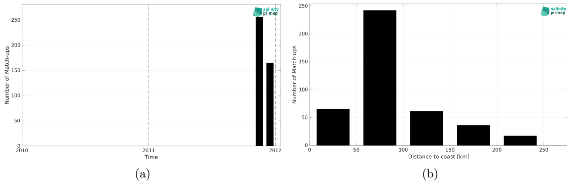
Figure 2: Number of match-ups between TSG (SAMOS) and CCI SSS L4 Merged-OI v4.41 - 30-day running (ESA) SSS as a function of time (a) and as function of the distance to coast (b) over the Mediterranean Sea Pi-MEP region and for the full satellite product period.
