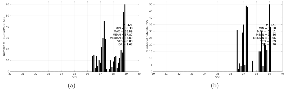
Figure 3: Histograms of SSS from TSG (SAMOS) (a) and CCI SSS L4 Merged-OI v4.41 - 30-day running (ESA) (b) considering all match-up pairs per bins of 0.1 over the Mediterranean Sea Pi-MEP region and for the full satellite product period.
