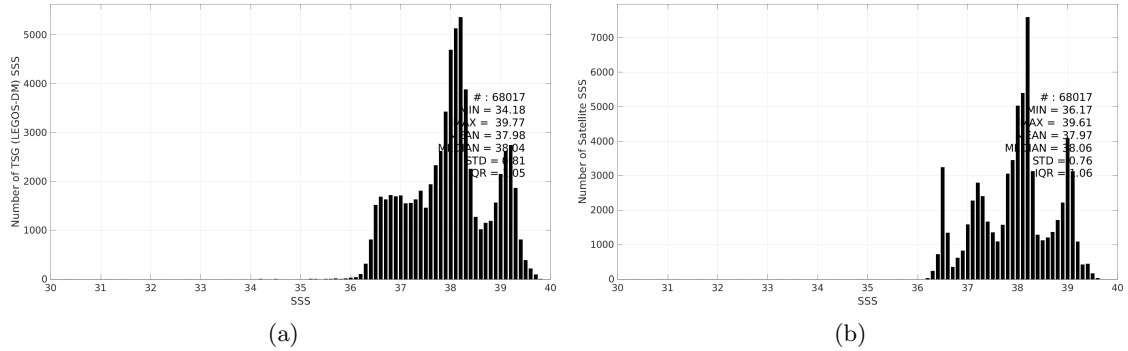
Figure 3: Histograms of SSS from TSG (LEGOS-DM) (a) and CCI SSS L4 Merged-OI v4.41 - 30-day running (ESA) (b) considering all match-up pairs per bins of 0.1 over the Mediterranean Sea Pi-MEP region and for the full satellite product period.
