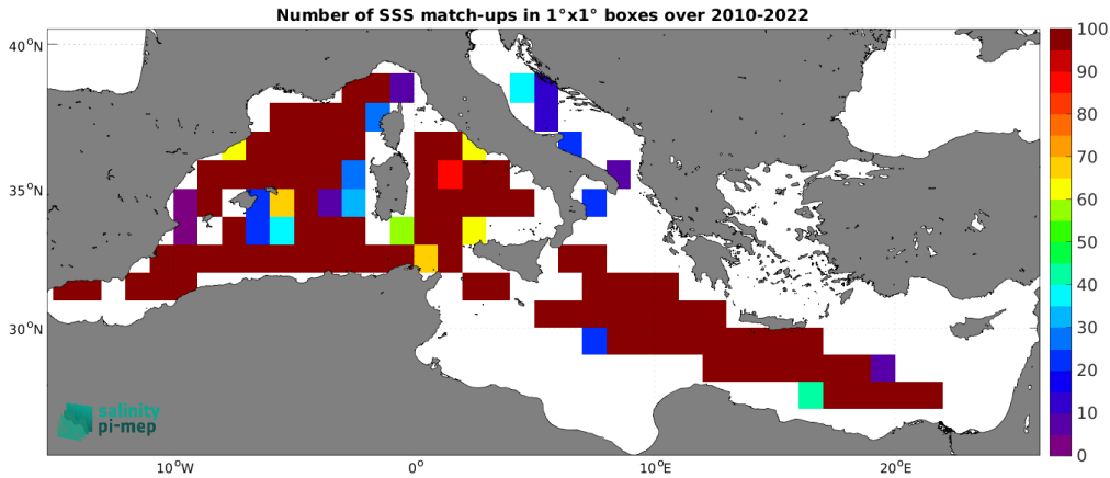
Figure 5: Number of SSS match-ups between TSG (LEGOS-DM) SSS and the CCI SSS L4 Merged-OI v4.41 - 30-day running (ESA) SSS product for the Mediterranean Sea Pi-MEP region over 1^\circ \times 1^\circ boxes and for the full satellite product period.
