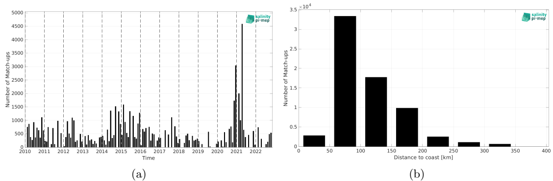
Figure 2: Number of match-ups between TSG (LEGOS-DM) and CCI SSS L4 Merged-OI v4.41 - 30-day running (ESA) SSS as a function of time (a) and as function of the distance to coast (b) over the Mediterranean Sea Pi-MEP region and for the full satellite product period.
