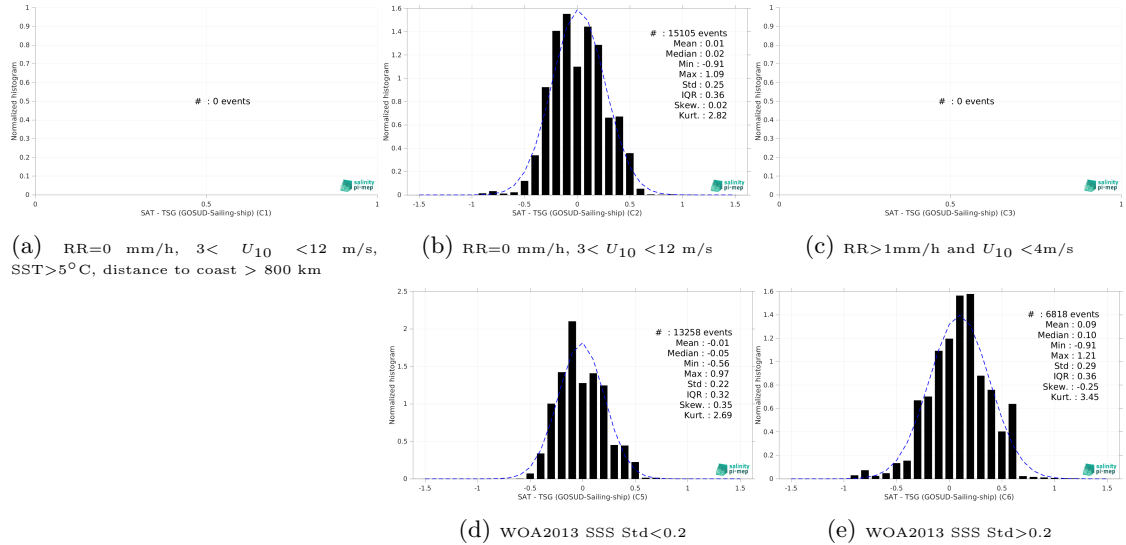
Figure 15: Normalized histogram of \Delta SSS (CCI SSS L4 Merged-OI v4.41 - 30-day running (ESA) - TSG (GOSUD-Sailing-ship)) for 5 different subdatasets corresponding to: RR=0 mm/h, 3 < U_{10} < 12 m/s, SST > 5°C, distance to coast > 800 km (a), RR=0 mm/h, 3 < U_{10} < 12 m/s (b), RR > 1mm/h and U_{10} < 4 m/s (c), WOA2013 SSS Std < 0.2 (d), WOA2013 SSS Std > 0.2 (e).
