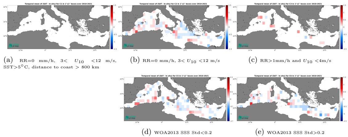
Figure 14: Temporal mean gridded over spatial boxes of size 1^\circ \times 1^\circ of \Delta SSS (CCI SSS L4 Merged-OI v4.41 - 30-day running (ESA) - TSG (GOSUD-Research-vessel)) for 5 different subdatasets corresponding to:RR=0 mm/h, 3 < U_{10} < 12 m/s, SST >5^\circ C, distance to coast > 800 km (a), RR=0 mm/h, 3 < U_{10} < 12 m/s (b), RR >1 mm/h and U_{10} < 4 m/s (c), WOA2013 SSS Std <0.2 (d), WOA2013 SSS Std >0.2 (e).
