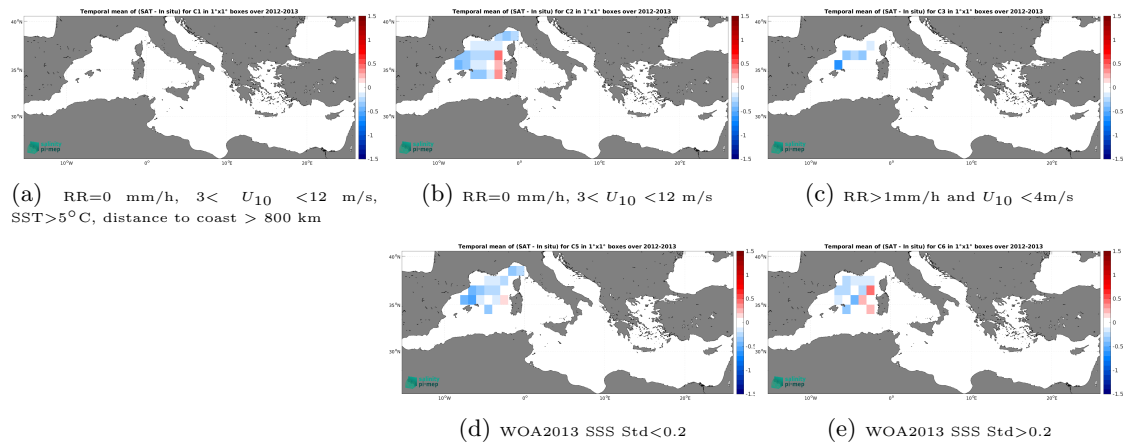
Figure 13: Temporal mean gridded over spatial boxes of size 1^\circ \times 1^\circ of \Delta\text{SSS} (CCI SSS L4 Merged-OI v4.41 - 30-day running (ESA) - Surface drifters) for 5 different subdatasets corresponding to:RR=0 mm/h, 3 < U_{10} < 12 m/s, SST >5^\circ\text{C} , distance to coast > 800 km (a), RR=0 mm/h, 3 < U_{10} < 12 m/s (b), RR >1 mm/h and U_{10} < 4 m/s (c), WOA2013 SSS Std <0.2 (d), WOA2013 SSS Std >0.2 (e).
