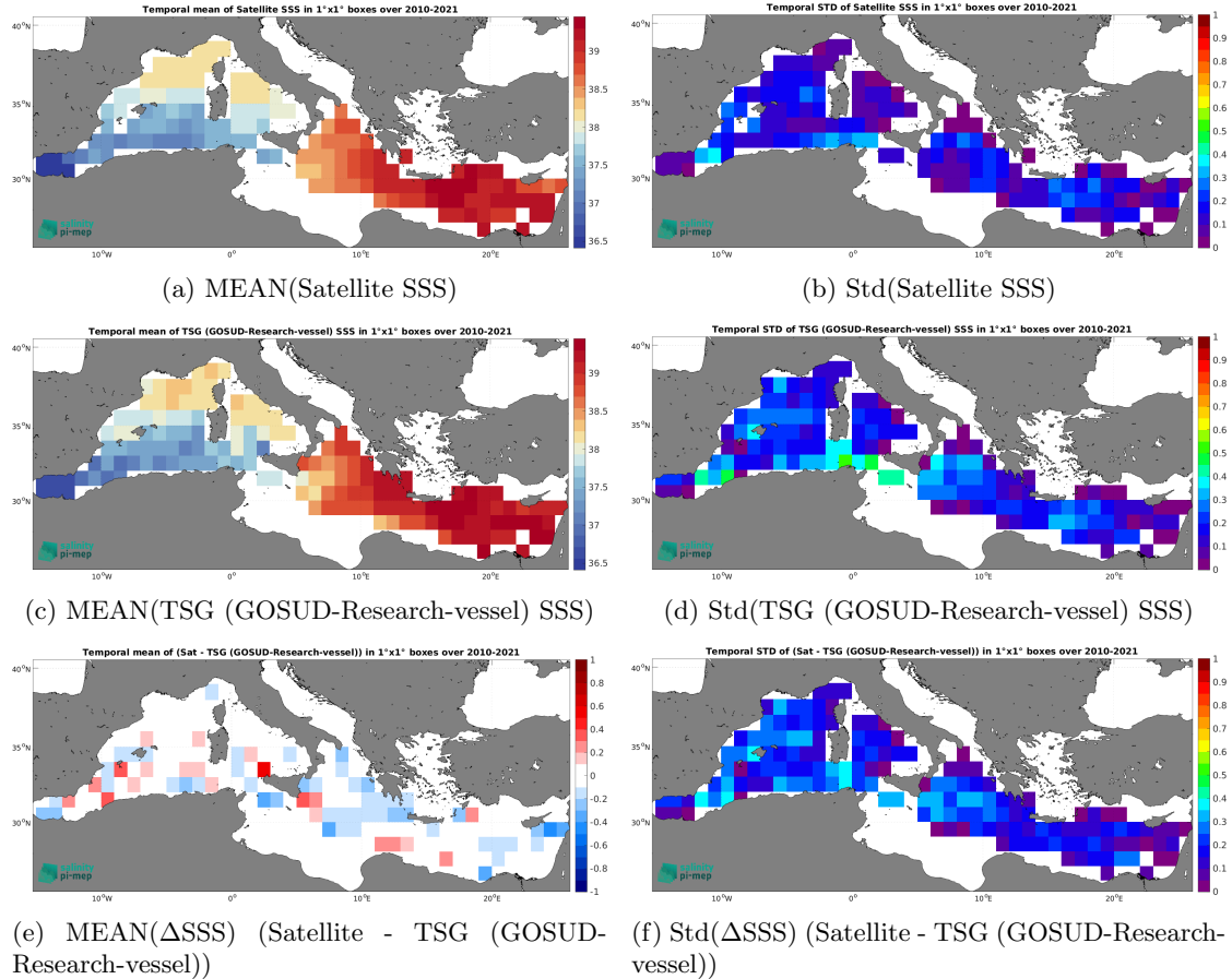
Figure 6: Temporal mean (left) and Std (right) of SSS from CCI SSS L4 Merged-OI v4.4 - 7-day running (ESA) (top), TSG (GOSUD-Research-vessel) (middle), and of \Delta\text{SSS} (Satellite - TSG (GOSUD-Research-vessel)). Only match-up pairs are used to generate these maps.
