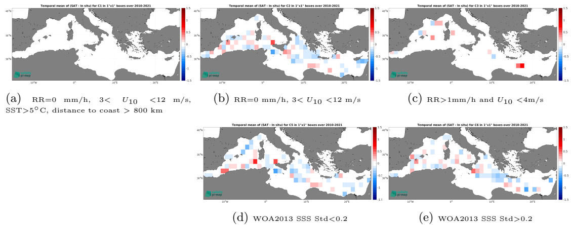
Figure 12: Temporal mean gridded over spatial boxes of size 1^{\circ}\times 1^{\circ} of \Delta SSS (CCI SSS L4 Merged-OI v4.4 - 7-day running (ESA) - TSG (GOSUD-Research-vessel)) for 5 different subdatasets corresponding to:RR=0 mm/h, 3 < U_{10} < 12 m/s, SST >5^{\circ}\text{C} , distance to coast > 800 km (a), RR=0 mm/h, 3 < U_{10} < 12 m/s (b), RR >1 mm/h and U_{10} < 4 m/s (c), WOA2013 SSS Std <0.2 (d), WOA2013 SSS Std >0.2 (e).
