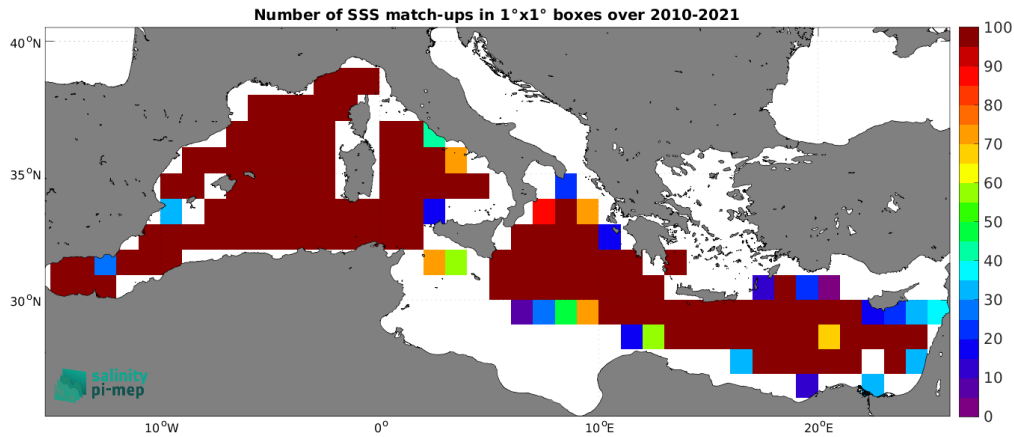
Figure 4: Number of SSS match-ups between TSG (GOSUD-Research-vessel) SSS and the CCI SSS L4 Merged-OI v4.4 - 7-day running (ESA) SSS product for the Mediterranean Sea Pi-MEP region over 1^\circ \times 1^\circ boxes and for the full satellite product period.
