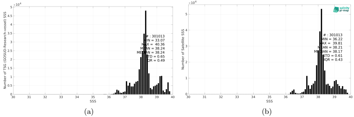
Figure 2: Histograms of SSS from TSG (GOSUD-Research-vessel) (a) and CCI SSS L4 Merged-OI v4.4 - 7-day running (ESA) (b) considering all match-up pairs per bins of 0.1 over the Mediterranean Sea Pi-MEP region and for the full satellite product period.
