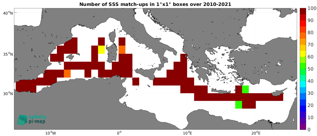
Figure 4: Number of SSS match-ups between TSG (CSIC-UTM) SSS and the CCI SSS L4 Merged-OI v4.4 - 7-day running (ESA) SSS product for the Mediterranean Sea Pi-MEP region over 1^\circ \times 1^\circ boxes and for the full satellite product period.
