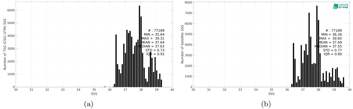
Figure 2: Histograms of SSS from TSG (CSIC-UTM) (a) and CCI SSS L4 Merged-OI v4.4 - 7-day running (ESA) (b) considering all match-up pairs per bins of 0.1 over the Mediterranean Sea Pi-MEP region and for the full satellite product period.
