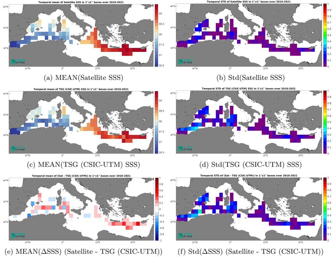
Figure 6: Temporal mean (left) and Std (right) of SSS from CCI SSS L4 Merged-OI v4.4 - 7-day running (ESA) (top), TSG (CSIC-UTM) (middle), and of \Delta\text{SSS} (Satellite - TSG (CSIC-UTM)). Only match-up pairs are used to generate these maps.
