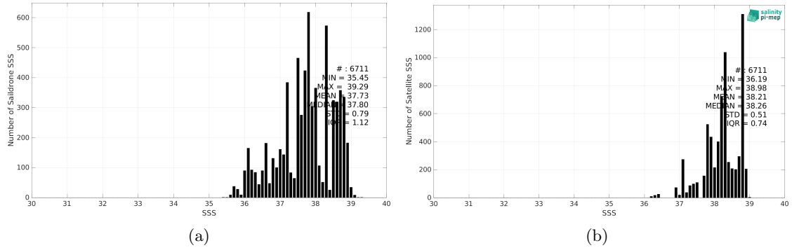
Figure 2: Histograms of SSS from Saildrone (a) and CCI SSS L4 Merged-OI v4.4 - 7-day running (ESA) (b) considering all match-up pairs per bins of 0.1 over the Mediterranean Sea Pi-MEP region and for the full satellite product period.
