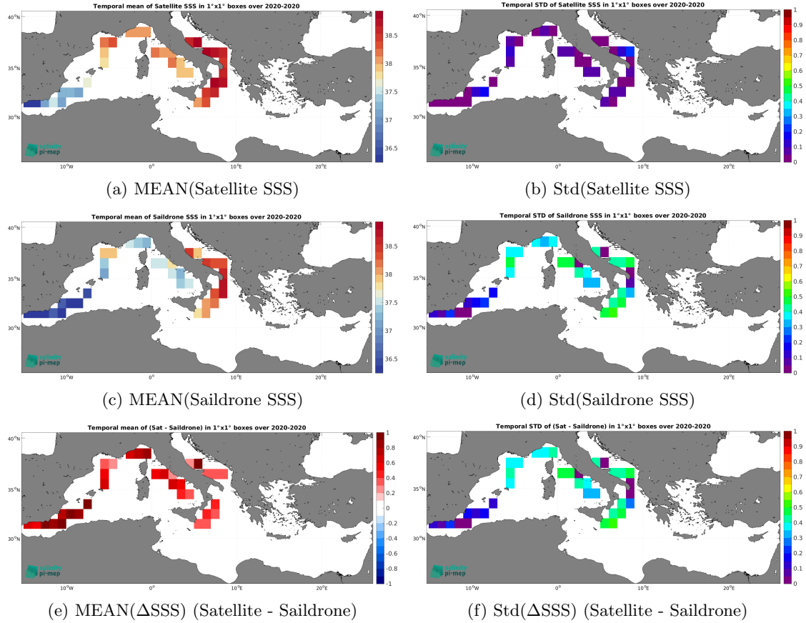
Figure 6: Temporal mean (left) and Std (right) of SSS from CCI SSS L4 Merged-OI v4.4 - 7-day running (ESA) (top), Saildrone (middle), and of \Delta\text{SSS} (Satellite - Saildrone). Only match-up pairs are used to generate these maps.
