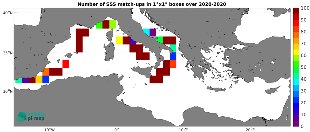
Figure 4: Number of SSS match-ups between Saildrone SSS and the CCI SSS L4 Merged-OI v4.4 - 7-day running (ESA) SSS product for the Mediterranean Sea Pi-MEP region over 1^\circ \times 1^\circ boxes and for the full satellite product period.
