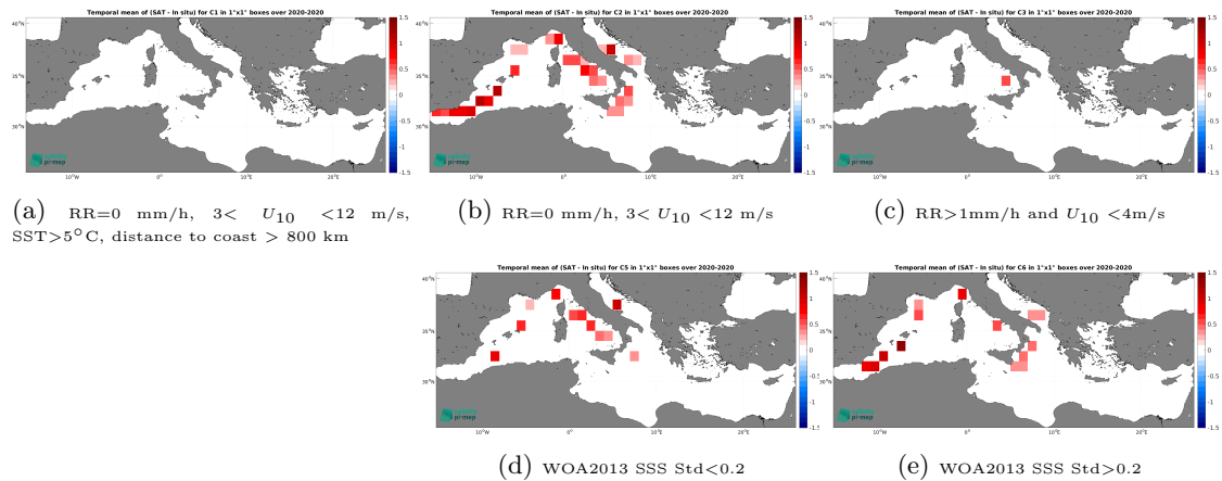
Figure 12: Temporal mean gridded over spatial boxes of size 1^\circ \times 1^\circ of \Delta SSS (CCI SSS L4 Merged-OI v4.4 - 7-day running (ESA) - Saildrone) for 5 different subdatasets corresponding to:RR=0 mm/h, 3 < U_{10} < 12 m/s, SST >5^\circ\text{C} , distance to coast > 800 km (a), RR=0 mm/h, 3 < U_{10} < 12 m/s (b), RR >1 mm/h and U_{10} < 4 m/s (c), WOA2013 SSS Std <0.2 (d), WOA2013 SSS Std >0.2 (e).
