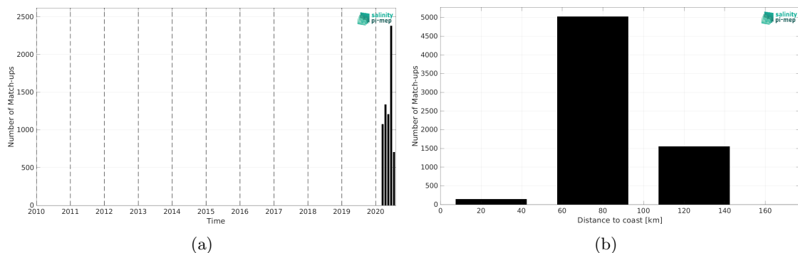
Figure 1: Number of match-ups between Saildrone and CCI SSS L4 Merged-OI v4.4 - 7-day running (ESA) SSS as a function of time (a) and as function of the distance to coast (b) over the Mediterranean Sea Pi-MEP region and for the full satellite product period.
