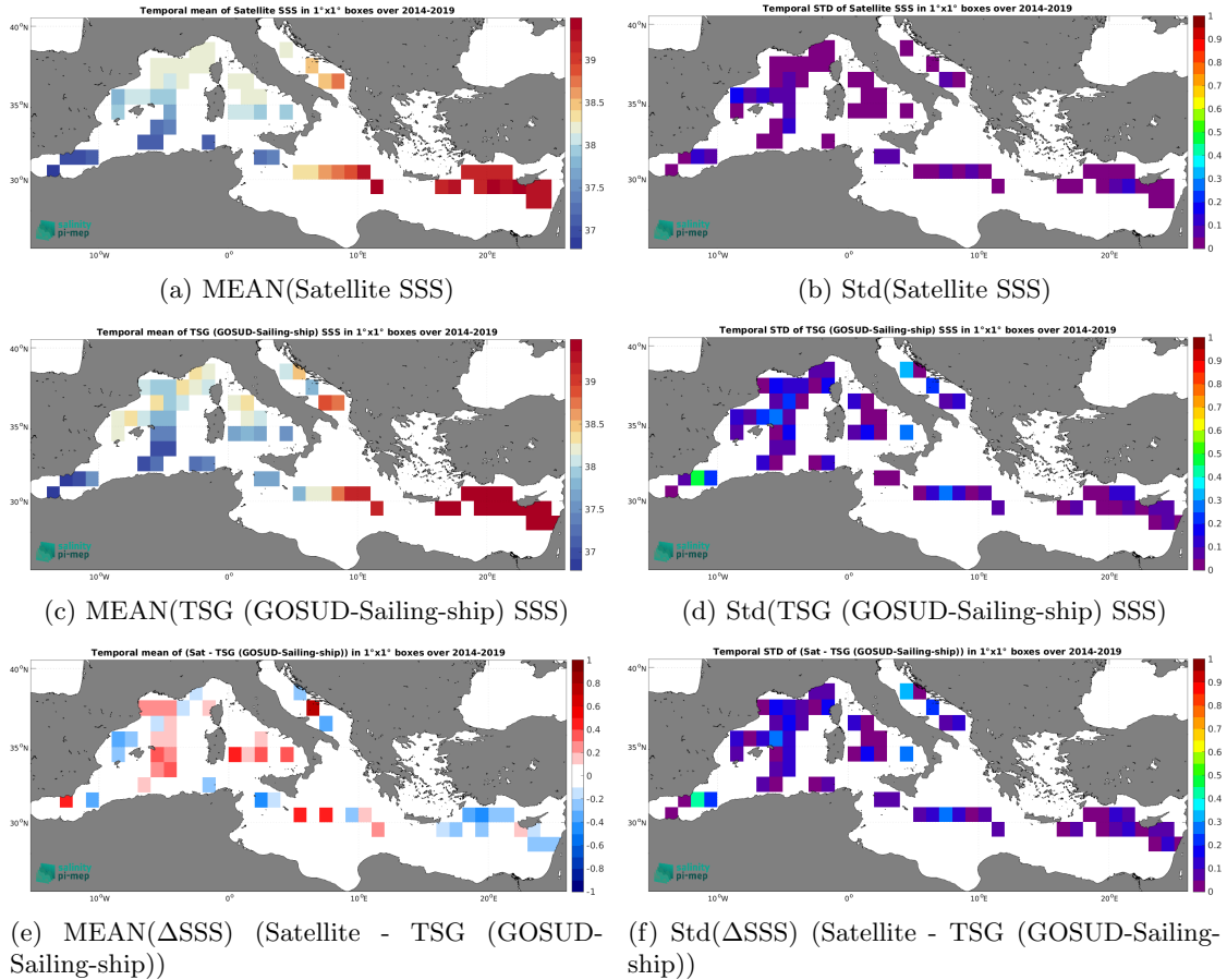
Figure 6: Temporal mean (left) and Std (right) of SSS from CCI SSS L4 Merged-OI v4.4 - 30-day running (ESA) (top), TSG (GOSUD-Sailing-ship) (middle), and of \Delta\text{SSS} (Satellite - TSG (GOSUD-Sailing-ship)). Only match-up pairs are used to generate these maps.
