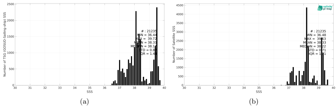
Figure 2: Histograms of SSS from TSG (GOSUD-Sailing-ship) (a) and CCI SSS L4 Merged-OI v4.4 - 30-day running (ESA) (b) considering all match-up pairs per bins of 0.1 over the Mediterranean Sea Pi-MEP region and for the full satellite product period.
