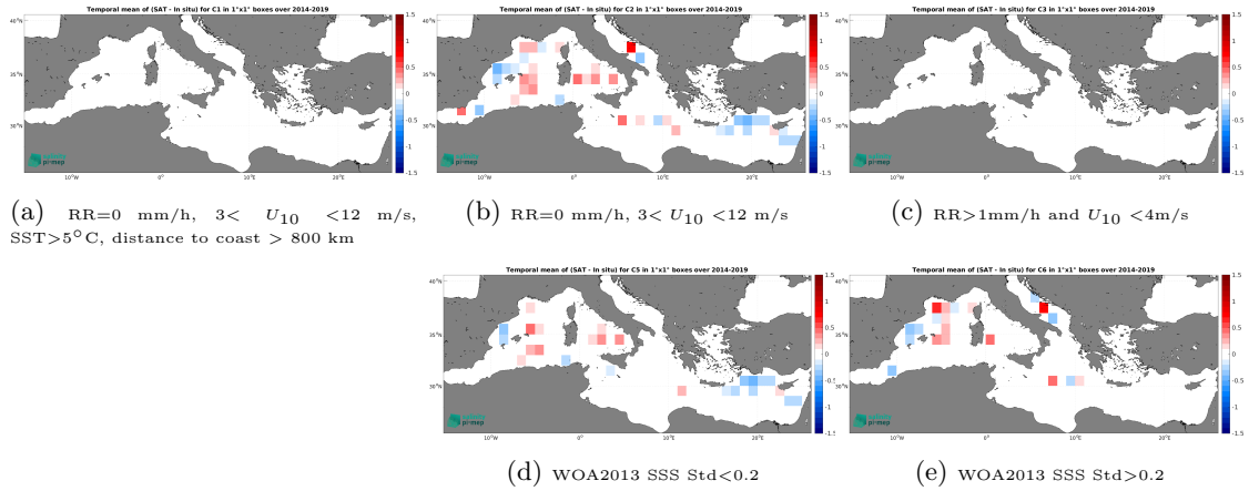
Figure 12: Temporal mean gridded over spatial boxes of size 1^{\circ}\times 1^{\circ} of \Delta SSS (CCI SSS L4 Merged-OI v4.4 - 30-day running (ESA) - TSG (GOSUD-Sailing-ship)) for 5 different subdatasets corresponding to:RR=0 mm/h, 3 < U_{10} < 12 m/s, SST >5^{\circ}\text{C} , distance to coast > 800 km (a), RR=0 mm/h, 3 < U_{10} < 12 m/s (b), RR >1 mm/h and U_{10} < 4 m/s (c), WOA2013 SSS Std <0.2 (d), WOA2013 SSS Std >0.2 (e).
