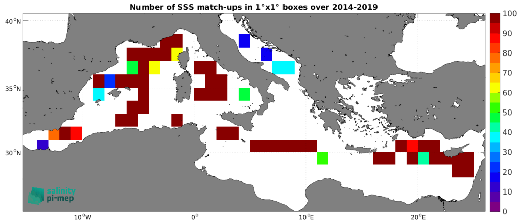
Figure 4: Number of SSS match-ups between TSG (GOSUD-Sailing-ship) SSS and the CCI SSS L4 Merged-OI v4.4 - 30-day running (ESA) SSS product for the Mediterranean Sea Pi-MEP region over 1^\circ \times 1^\circ boxes and for the full satellite product period.
