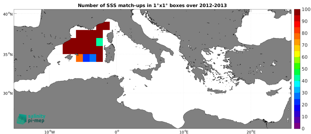
Figure 3: Number of SSS match-ups between Surface drifters SSS and the CCI SSS L4 Merged-OI v4.4 - 30-day running (ESA) SSS product for the Mediterranean Sea Pi-MEP region over 1^\circ \times 1^\circ boxes and for the full satellite product period.
