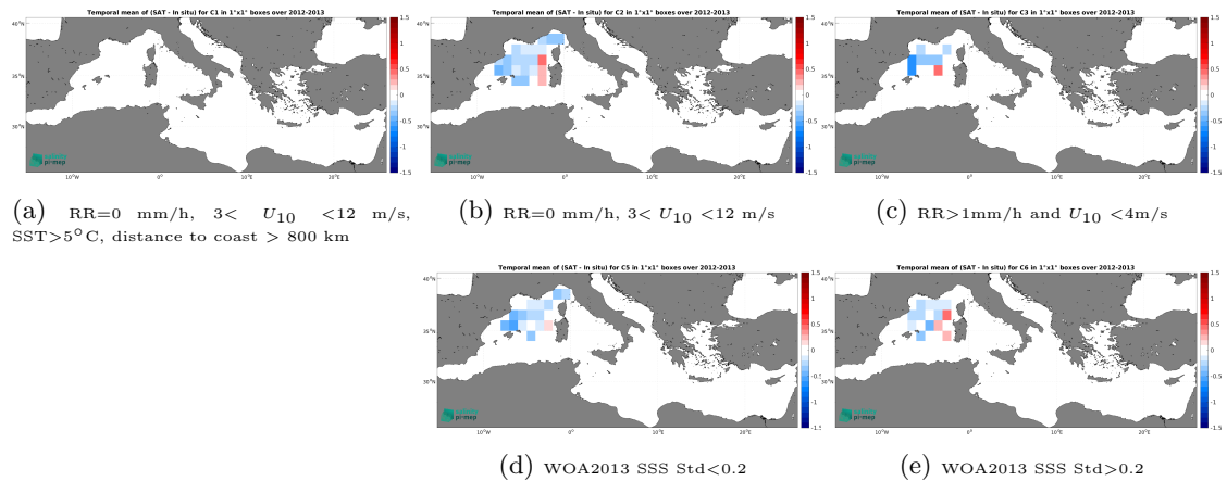
Figure 11: Temporal mean gridded over spatial boxes of size 1^\circ \times 1^\circ of \Delta SSS (CCI SSS L4 Merged-OI v4.4 - 30-day running (ESA) - Surface drifters) for 5 different subdatasets corresponding to:RR=0 mm/h, 3 < U_{10} < 12 m/s, SST >5^\circ C, distance to coast > 800 km (a), RR=0 mm/h, 3 < U_{10} < 12 m/s (b), RR >1 mm/h and U_{10} < 4 m/s (c), WOA2013 SSS Std <0.2 (d), WOA2013 SSS Std >0.2 (e).
