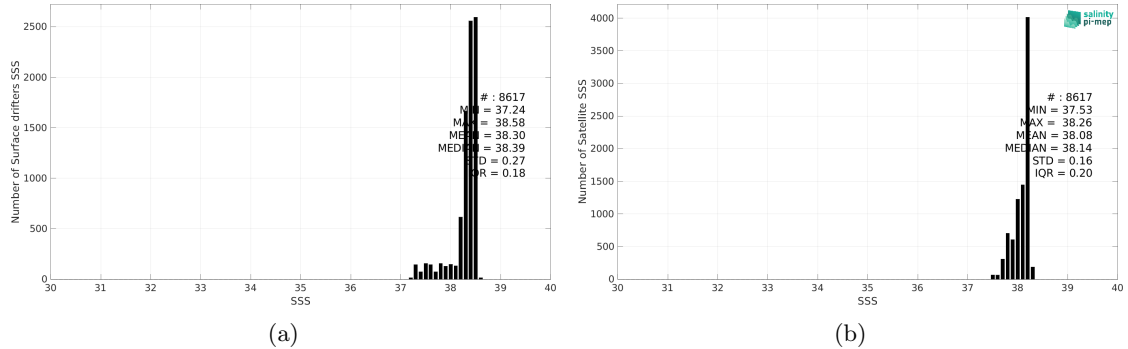
Figure 2: Histograms of SSS from Surface drifters (a) and CCI SSS L4 Merged-OI v4.4 - 30-day running (ESA) (b) considering all match-up pairs per bins of 0.1 over the Mediterranean Sea Pi-MEP region and for the full satellite product period.
