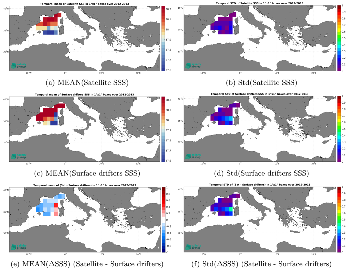
Figure 5: Temporal mean (left) and Std (right) of SSS from CCI SSS L4 Merged-OI v4.4 - 30-day running (ESA) (top), Surface drifters (middle), and of \Delta SSS (Satellite - Surface drifters). Only match-up pairs are used to generate these maps.
