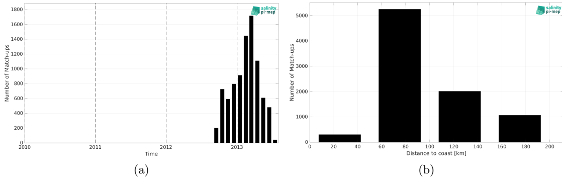
Figure 1: Number of match-ups between Surface drifters and CCI SSS L4 Merged-OI v4.4 - 30-day running (ESA) SSS as a function of time (a) and as function of the distance to coast (b) over the Mediterranean Sea Pi-MEP region and for the full satellite product period.
