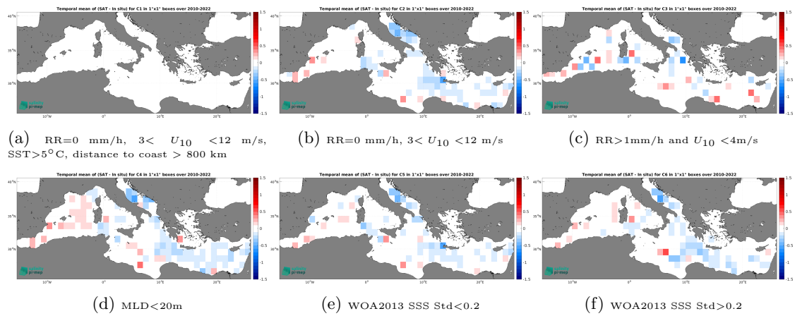
Figure 12: Temporal mean gridded over spatial boxes of size 1^\circ \times 1^\circ of \Delta SSS (CCI SSS L4 Merged-OI v4.4 - 30-day running (ESA) - Argo) for 6 different subdatasets corresponding to:RR=0 mm/h, 3 < U_{10} < 12 m/s, SST >5^\circ C, distance to coast > 800 km (a), RR=0 mm/h, 3 < U_{10} < 12 m/s (b), RR >1 mm/h and U_{10} < 4 m/s (c),MLD <20 m (d),WOA2013 SSS Std <0.2 (e),WOA2013 SSS Std >0.2 (f).
