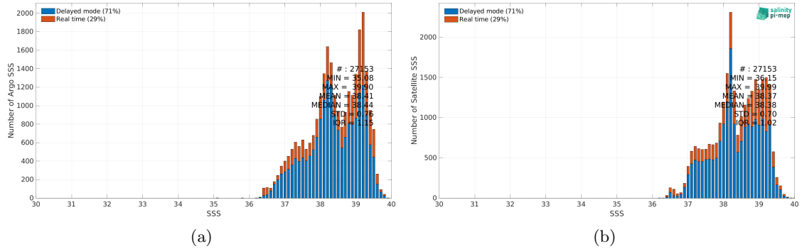
Figure 2: Histograms of SSS from Argo (a) and CCI SSS L4 Merged-OI v4.4 - 30-day running (ESA) (b) considering all match-up pairs per bins of 0.1 over the Mediterranean Sea Pi-MEP region and for the full satellite product period.
