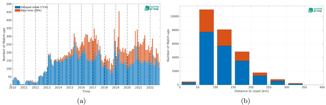
Figure 1: Number of match-ups between Argo and CCI SSS L4 Merged-OI v4.4 - 30-day running (ESA) SSS as a function of time (a) and as function of the distance to coast (b) over the Mediterranean Sea Pi-MEP region and for the full satellite product period.
