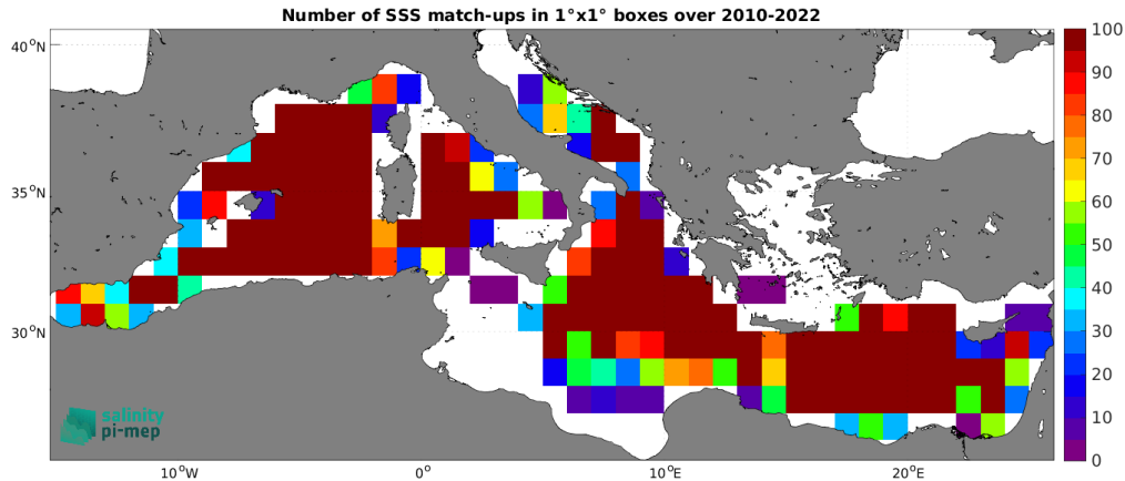
Figure 4: Number of SSS match-ups between Argo SSS and the CCI SSS L4 Merged-OI v4.4 - 30-day running (ESA) SSS product for the Mediterranean Sea Pi-MEP region over 1^\circ \times 1^\circ boxes and for the full satellite product period.
