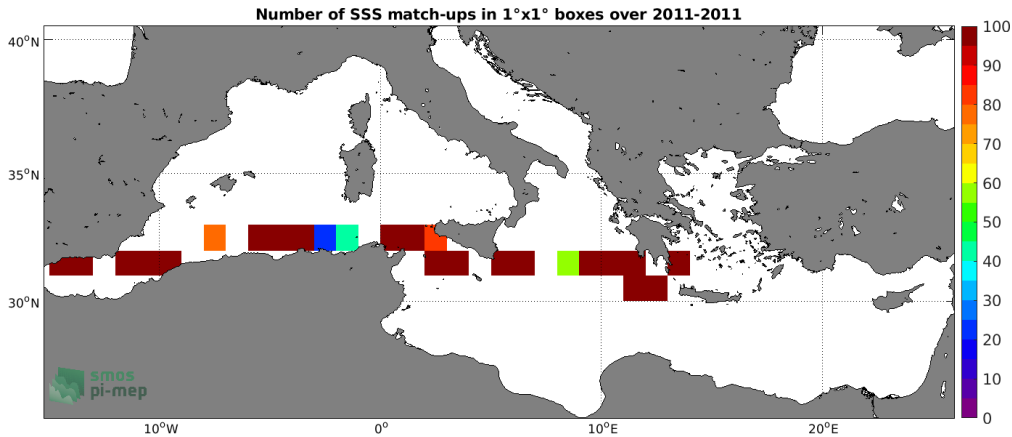
Figure 4: Number of SSS match-ups between TSG (SAMOS) SSS and the CCI SSS L4 Merged-OI v3.2 - 7-day running (ESA) SSS product for the Mediterranean Sea Pi-MEP region over 1°x1° boxes and for the full satellite product period.
