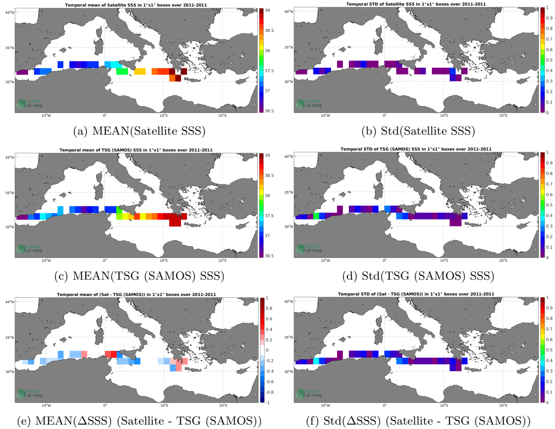
Figure 6: Temporal mean (left) and Std (right) of SSS from CCI SSS L4 Merged-OI v3.2 - 7-day running (ESA) (top), TSG (SAMOS) (middle), and of \Delta SSS (Satellite - TSG (SAMOS)). Only match-up pairs are used to generate these maps.
