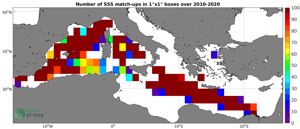
Figure 4: Number of SSS match-ups between TSG (LEGOS-DM) SSS and the CCI SSS L4 Merged-OI v3.2 - 7-day running (ESA) SSS product for the Mediterranean Sea Pi-MEP region over 1°x1° boxes and for the full satellite product period.
