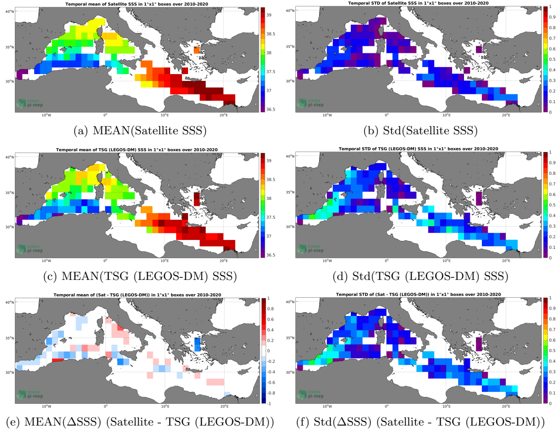
Figure 6: Temporal mean (left) and Std (right) of SSS from CCI SSS L4 Merged-OI v3.2 - 7-day running (ESA) (top), TSG (LEGOS-DM) (middle), and of \Delta SSS (Satellite - TSG (LEGOS-DM)). Only match-up pairs are used to generate these maps.
