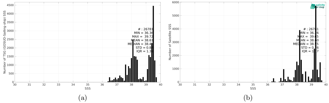
Figure 2: Histograms of SSS from TSG (GOSUD-Sailing-ship) (a) and CCI SSS L4 Merged-OI v3.2 - 7-day running (ESA) (b) considering all match-up pairs per bins of 0.1 over the Mediterranean Sea Pi-MEP region and for the full satellite product period.
