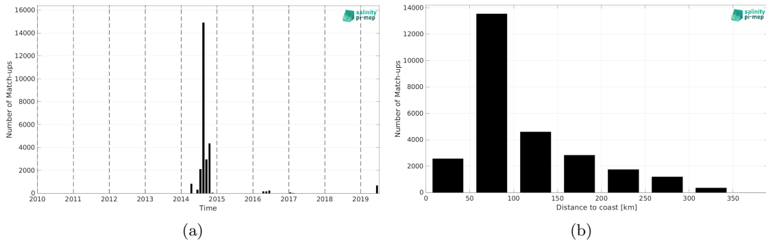
Figure 1: Number of match-ups between TSG (GOSUD-Sailing-ship) and CCI SSS L4 Merged-OI v3.2 - 7-day running (ESA) SSS as a function of time (a) and as function of the distance to coast (b) over the Mediterranean Sea Pi-MEP region and for the full satellite product period.
