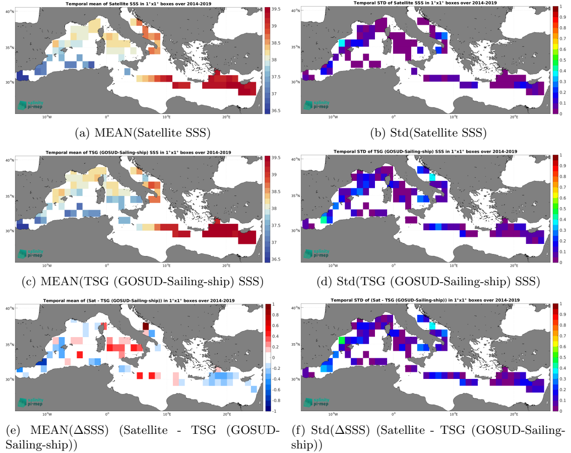
Figure 6: Temporal mean (left) and Std (right) of SSS from CCI SSS L4 Merged-OI v3.2 - 7-day running (ESA) (top), TSG (GOSUD-Sailing-ship) (middle), and of \Delta\text{SSS} (Satellite - TSG (GOSUD-Sailing-ship)). Only match-up pairs are used to generate these maps.
