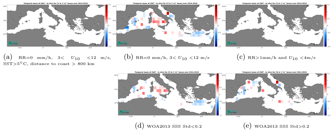
Figure 12: Temporal mean gridded over spatial boxes of size 1^\circ \times 1^\circ of \Delta SSS (CCI SSS L4 Merged-OI v3.2 - 7-day running (ESA) - TSG (GOSUD-Sailing-ship)) for 5 different subdatasets corresponding to:RR=0 mm/h, 3 < U_{10} < 12 m/s, SST >5^\circ\text{C} , distance to coast > 800 km (a), RR=0 mm/h, 3 < U_{10} < 12 m/s (b), RR >1 mm/h and U_{10} < 4 m/s (c), WOA2013 SSS Std <0.2 (d), WOA2013 SSS Std >0.2 (e).
