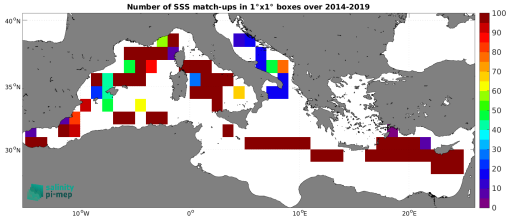
Figure 4: Number of SSS match-ups between TSG (GOSUD-Sailing-ship) SSS and the CCI SSS L4 Merged-OI v3.2 - 7-day running (ESA) SSS product for the Mediterranean Sea Pi-MEP region over 1^\circ \times 1^\circ boxes and for the full satellite product period.
