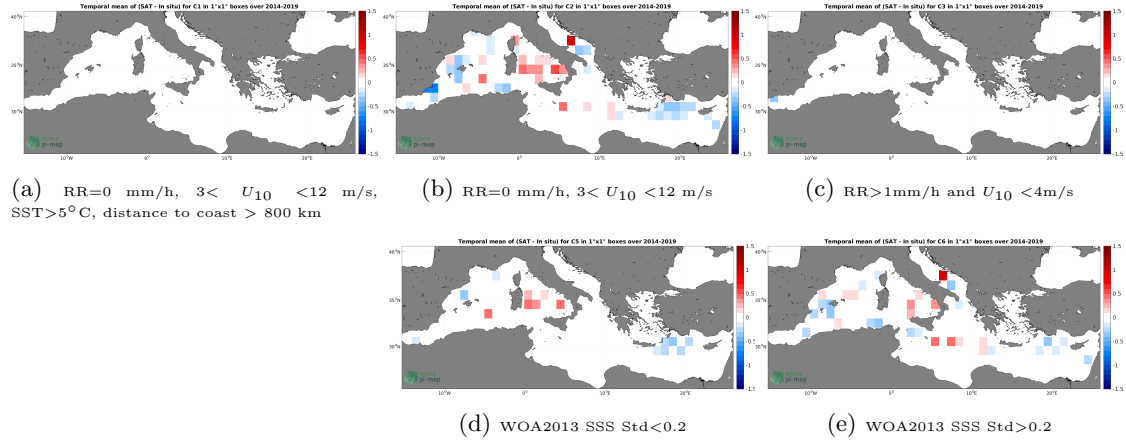
Figure 12: Temporal mean gridded over spatial boxes of size 1^{\circ}\times 1^{\circ} of \Delta SSS (CCI SSS L4 Merged-OI v3.2 - 7-day running (ESA) - TSG (GOSUD-Sailing-ship)) for 5 different subdatasets corresponding to:RR=0 mm/h, 3 < U_{10} < 12 m/s, SST >5^{\circ}\text{C} , distance to coast > 800 km (a), RR=0 mm/h, 3 < U_{10} < 12 m/s (b), RR >1 mm/h and U_{10} < 4 m/s (c), WOA2013 SSS Std <0.2 (d), WOA2013 SSS Std >0.2 (e).
