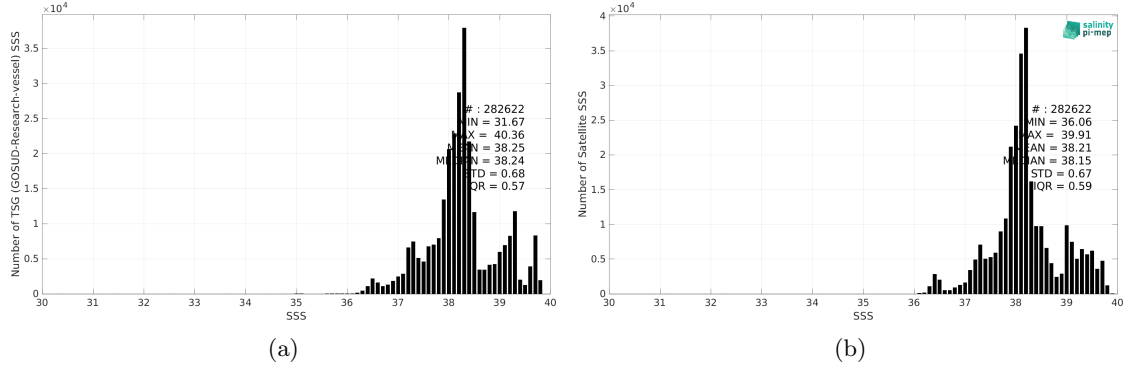
Figure 2: Histograms of SSS from TSG (GOSUD-Research-vessel) (a) and CCI SSS L4 Merged-OI v3.2 - 7-day running (ESA) (b) considering all match-up pairs per bins of 0.1 over the Mediterranean Sea Pi-MEP region and for the full satellite product period.
