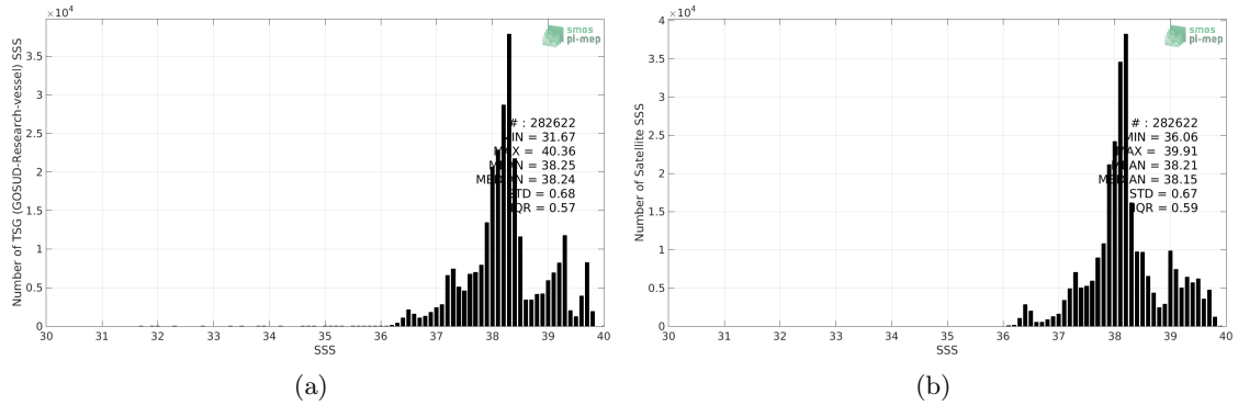
Figure 2: Histograms of SSS from TSG (GOSUD-Research-vessel) (a) and CCI SSS L4 Merged-OI v3.2 - 7-day running (ESA) (b) considering all match-up pairs per bins of 0.1 over the Mediterranean Sea Pi-MEP region and for the full satellite product period.
