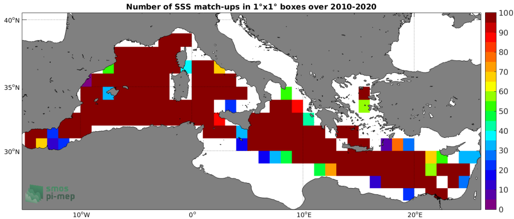
Figure 4: Number of SSS match-ups between TSG (GOSUD-Research-vessel) SSS and the CCI SSS L4 Merged-OI v3.2 - 7-day running (ESA) SSS product for the Mediterranean Sea Pi-MEP region over 1^\circ \times 1^\circ boxes and for the full satellite product period.
