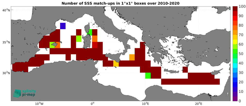
Figure 4: Number of SSS match-ups between TSG (CSIC-UTM) SSS and the CCI SSS L4 Merged-OI v3.2 - 7-day running (ESA) SSS product for the Mediterranean Sea Pi-MEP region over 1^\circ \times 1^\circ boxes and for the full satellite product period.
