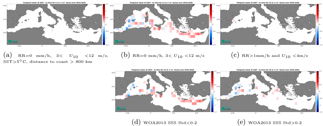
Figure 12: Temporal mean gridded over spatial boxes of size 1^\circ \times 1^\circ of \Delta SSS (CCI SSS L4 Merged-OI v3.2 - 7-day running (ESA) - TSG (CSIC-UTM)) for 5 different subdatasets corresponding to:RR=0 mm/h, 3 < U_{10} < 12 m/s, SST >5^\circ\text{C} , distance to coast > 800 km (a), RR=0 mm/h, 3 < U_{10} < 12 m/s (b), RR >1 mm/h and U_{10} < 4 m/s (c), WOA2013 SSS Std <0.2 (d), WOA2013 SSS Std >0.2 (e).
