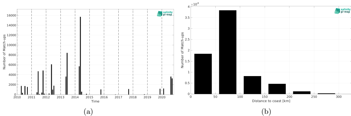
Figure 1: Number of match-ups between TSG (CSIC-UTM) and CCI SSS L4 Merged-OI v3.2 - 7-day running (ESA) SSS as a function of time (a) and as function of the distance to coast (b) over the Mediterranean Sea Pi-MEP region and for the full satellite product period.
