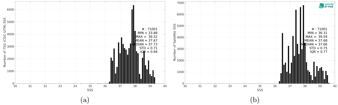
Figure 2: Histograms of SSS from TSG (CSIC-UTM) (a) and CCI SSS L4 Merged-OI v3.2 - 7-day running (ESA) (b) considering all match-up pairs per bins of 0.1 over the Mediterranean Sea Pi-MEP region and for the full satellite product period.
