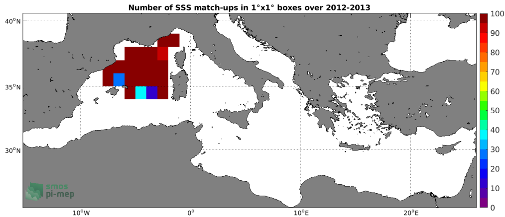
Figure 3: Number of SSS match-ups between Surface drifters SSS and the CCI SSS L4 Merged-OI v3.2 - 7-day running (ESA) SSS product for the Mediterranean Sea Pi-MEP region over 1^\circ \times 1^\circ boxes and for the full satellite product period.
