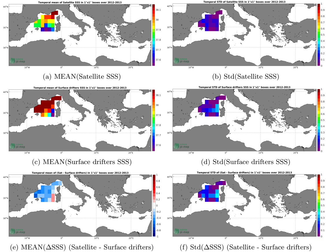
Figure 5: Temporal mean (left) and Std (right) of SSS from CCI SSS L4 Merged-OI v3.2 - 7-day running (ESA) (top), Surface drifters (middle), and of \Delta SSS (Satellite - Surface drifters). Only match-up pairs are used to generate these maps.
