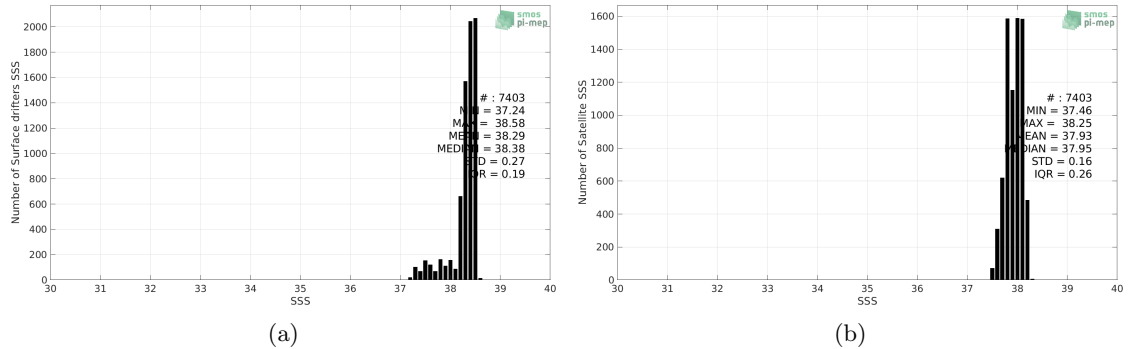
Figure 2: Histograms of SSS from Surface drifters (a) and CCI SSS L4 Merged-OI v3.2 - 7-day running (ESA) (b) considering all match-up pairs per bins of 0.1 over the Mediterranean Sea Pi-MEP region and for the full satellite product period.
