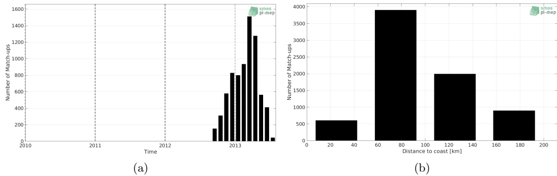
Figure 1: Number of match-ups between Surface drifters and CCI SSS L4 Merged-OI v3.2 - 7-day running (ESA) SSS as a function of time (a) and as function of the distance to coast (b) over the Mediterranean Sea Pi-MEP region and for the full satellite product period.
