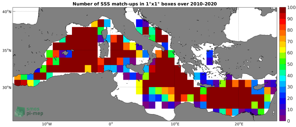
Figure 4: Number of SSS match-ups between Argo SSS and the CCI SSS L4 Merged-OI v3.2 - 7-day running (ESA) SSS product for the Mediterranean Sea Pi-MEP region over 1^\circ \times 1^\circ boxes and for the full satellite product period.
