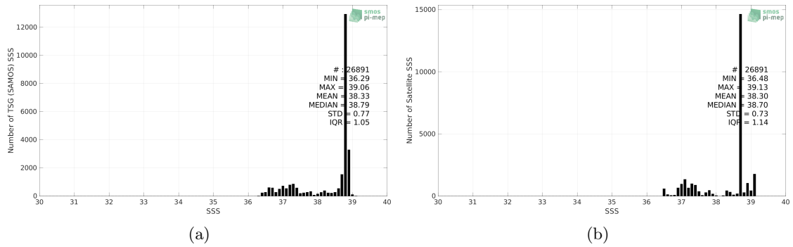
Figure 2: Histograms of SSS from TSG (SAMOS) (a) and CCI SSS L4 Merged-OI v3.2 - 30-day running (ESA) (b) considering all match-up pairs per bins of 0.1 over the Mediterranean Sea Pi-MEP region and for the full satellite product period.
