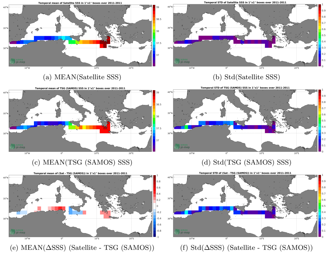
Figure 6: Temporal mean (left) and Std (right) of SSS from CCI SSS L4 Merged-OI v3.2 - 30-day running (ESA) (top), TSG (SAMOS) (middle), and of \Delta SSS (Satellite - TSG (SAMOS)). Only match-up pairs are used to generate these maps.
