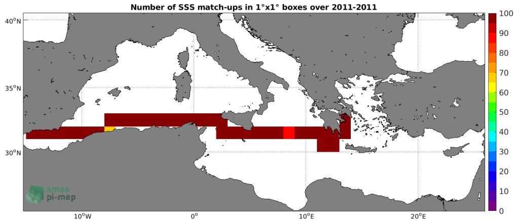
Figure 4: Number of SSS match-ups between TSG (SAMOS) SSS and the CCI SSS L4 Merged-OI v3.2 - 30-day running (ESA) SSS product for the Mediterranean Sea Pi-MEP region over 1°x1° boxes and for the full satellite product period.
