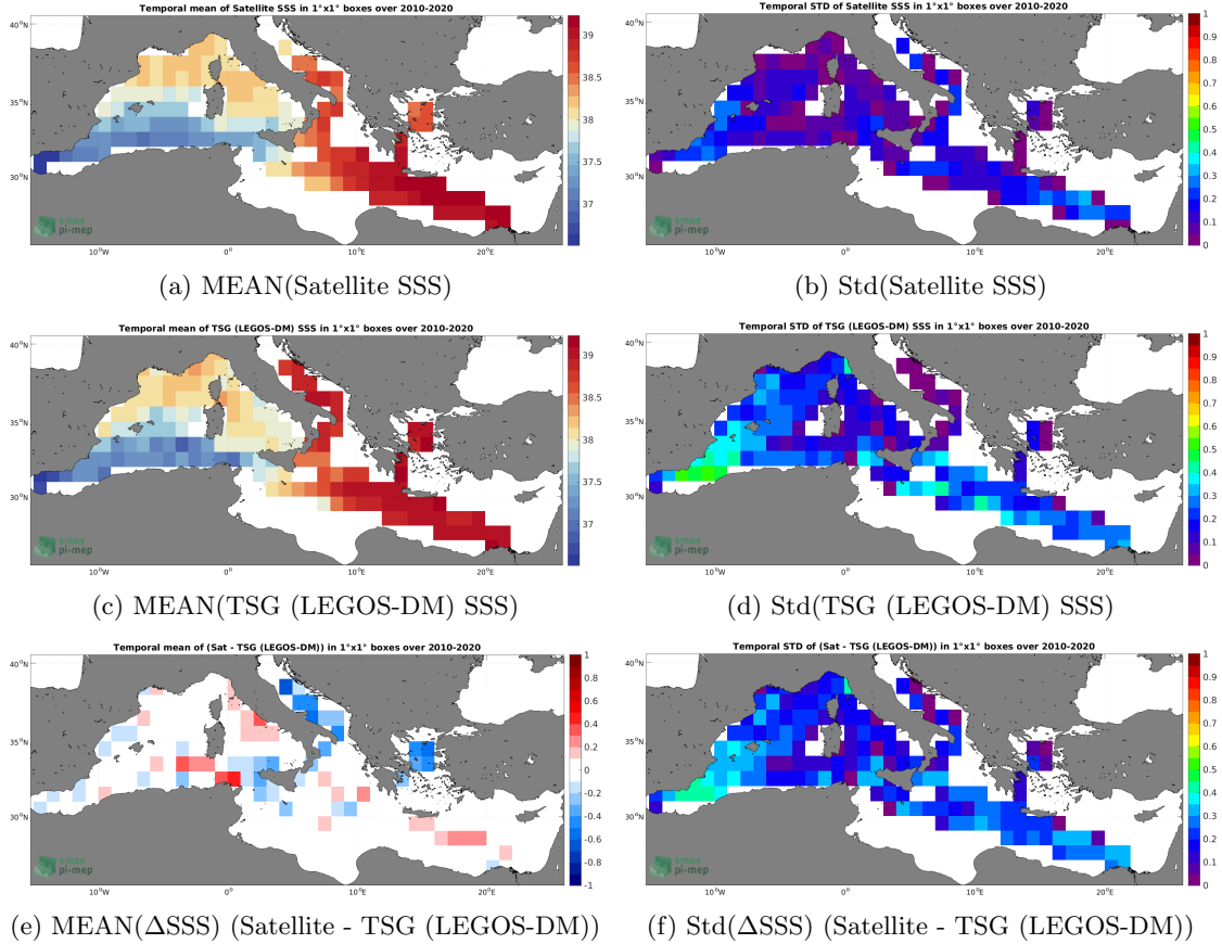
Figure 6: Temporal mean (left) and Std (right) of SSS from CCI SSS L4 Merged-OI v3.2 - 30-day running (ESA) (top), TSG (LEGOS-DM) ( in situ ) dataset (middle), and of \Delta\text{SSS} (Satellite - TSG (LEGOS-DM)). Only match-up pairs are used to generate these maps.
