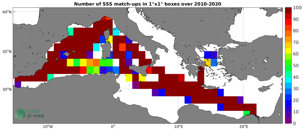
Figure 4: Number of SSS match-ups between TSG (LEGOS-DM) SSS and the CCI SSS L4 Merged-OI v3.2 - 30-day running (ESA) SSS product for the Mediterranean Sea Pi-MEP region over 1^\circ \times 1^\circ boxes and for the full satellite product period.
