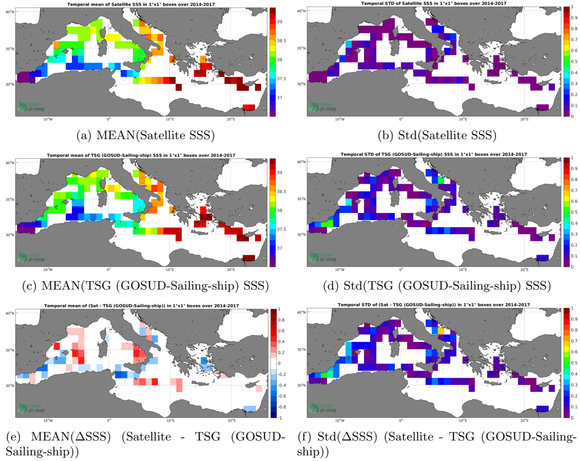
Figure 6: Temporal mean (left) and Std (right) of SSS from CCI SSS L4 Merged-OI v3.2 - 30-day running (ESA) (top), TSG (GOSUD-Sailing-ship) (middle), and of \Delta SSS (Satellite - TSG (GOSUD-Sailing-ship)). Only match-up pairs are used to generate these maps.
