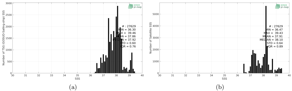
Figure 2: Histograms of SSS from TSG (GOSUD-Sailing-ship) (a) and CCI SSS L4 Merged-OI v3.2 - 30-day running (ESA) (b) considering all match-up pairs per bins of 0.1 over the Mediterranean Sea Pi-MEP region and for the full satellite product period.
