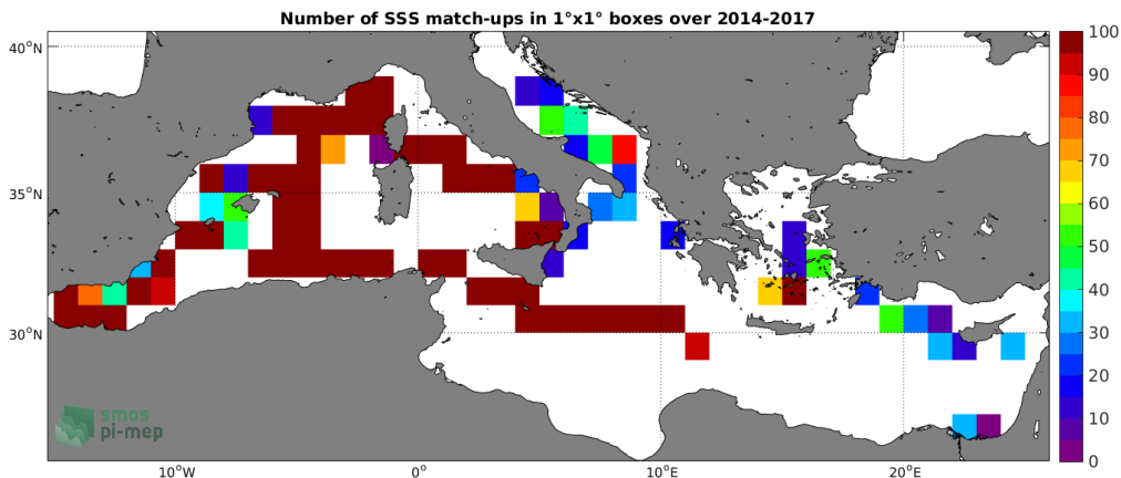
Figure 4: Number of SSS match-ups between TSG (GOSUD-Sailing-ship) SSS and the CCI SSS L4 Merged-OI v3.2 - 30-day running (ESA) SSS product for the Mediterranean Sea Pi-MEP region over 1°x1° boxes and for the full satellite product period.
