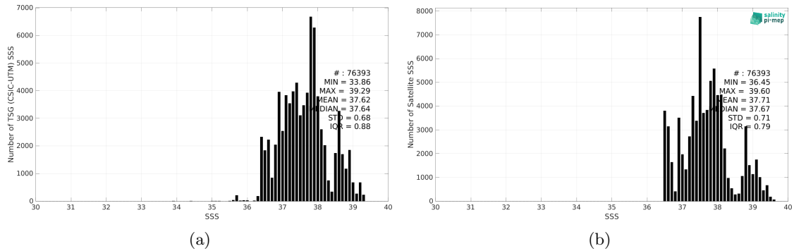
Figure 2: Histograms of SSS from TSG (CSIC-UTM) (a) and CCI SSS L4 Merged-OI v3.2 - 30-day running (ESA) (b) considering all match-up pairs per bins of 0.1 over the Mediterranean Sea Pi-MEP region and for the full satellite product period.
