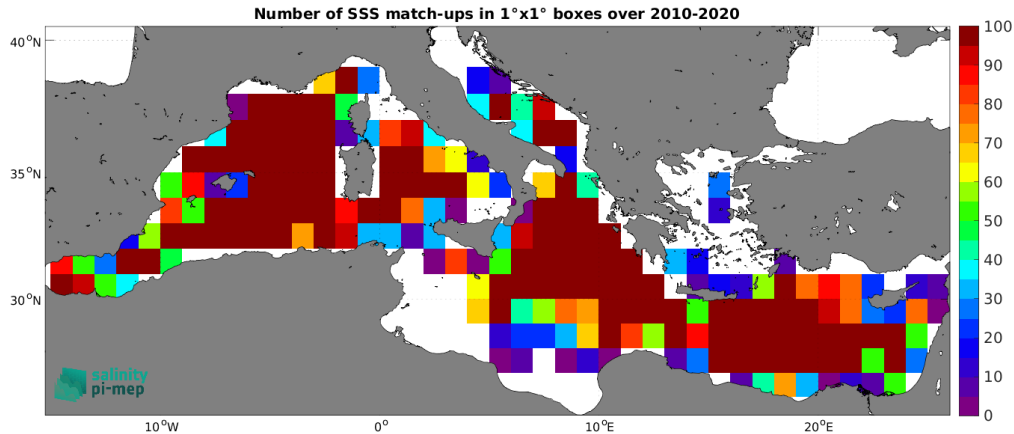
Figure 4: Number of SSS match-ups between Argo SSS and the CCI SSS L4 Merged-OI v3.2 - 30-day running (ESA) SSS product for the Mediterranean Sea Pi-MEP region over 1^\circ \times 1^\circ boxes and for the full satellite product period.
