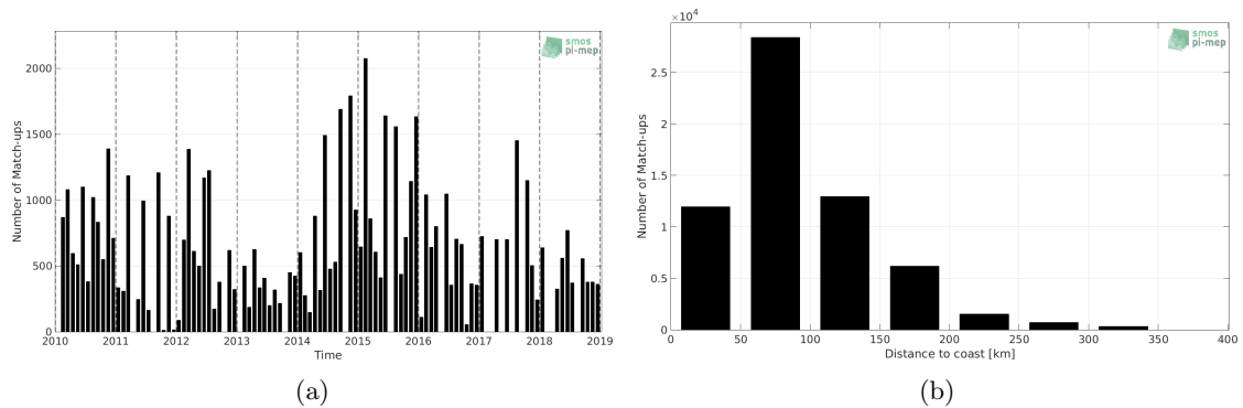
Figure 1: Number of match-ups between TSG (LEGOS-DM) and CCI SSS L4 Merged-OI v2.31 - 7-day running (ESA) SSS as a function of time (a) and as function of the distance to coast (b) over the Mediterranean Sea Pi-MEP region and for the full satellite product period.
