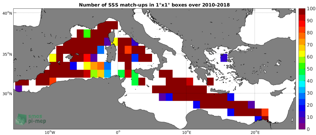
Figure 4: Number of SSS match-ups between TSG (LEGOS-DM) SSS and the CCI SSS L4 Merged-OI v2.31 - 7-day running (ESA) SSS product for the Mediterranean Sea Pi-MEP region over 1^\circ \times 1^\circ boxes and for the full satellite product period.
