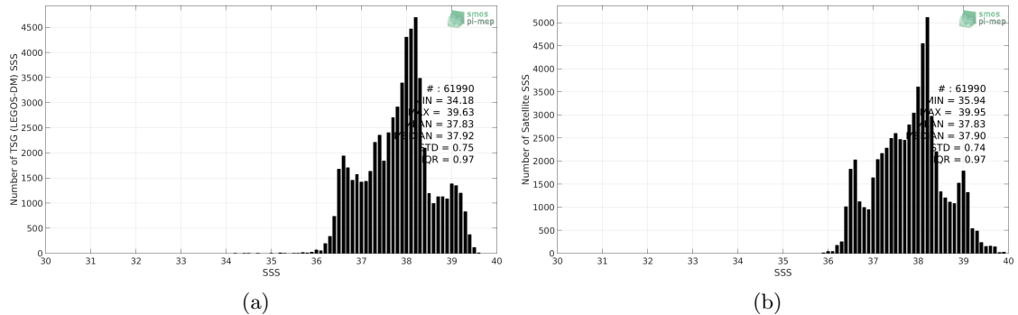
Figure 2: Histograms of SSS from TSG (LEGOS-DM) (a) and CCI SSS L4 Merged-OI v2.31 - 7-day running (ESA) (b) considering all match-up pairs per bins of 0.1 over the Mediterranean Sea Pi-MEP region and for the full satellite product period.
